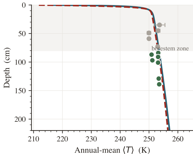
(c) Apollo 15 — deep-sensor zoom
