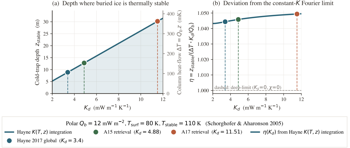
Figure 10. Polar cold-trap depth vs. K_d (Schorghofer-2005-style estimate at T_{\text{surf}} = 80 \text{ K} , Q_b = 12 \text{ mW/m}^2 ). (a) z_{\text{stable}} from forward-integrating dT/dz = Q_b/K(T, z) through the Hayne profile until T = T_{\text{stable}} = 110 \text{ K} ; right axis recasts the same depth as the column heat-flow drop \Delta T = Q_b z . (b) Ratio \eta = z_{\text{stable}}/[(\Delta T) K_d/Q_b] relative to the constant- K Fourier limit; \eta \approx 1.04 – 1.05 quantifies the shallow- K_s + radiative-term correction.
