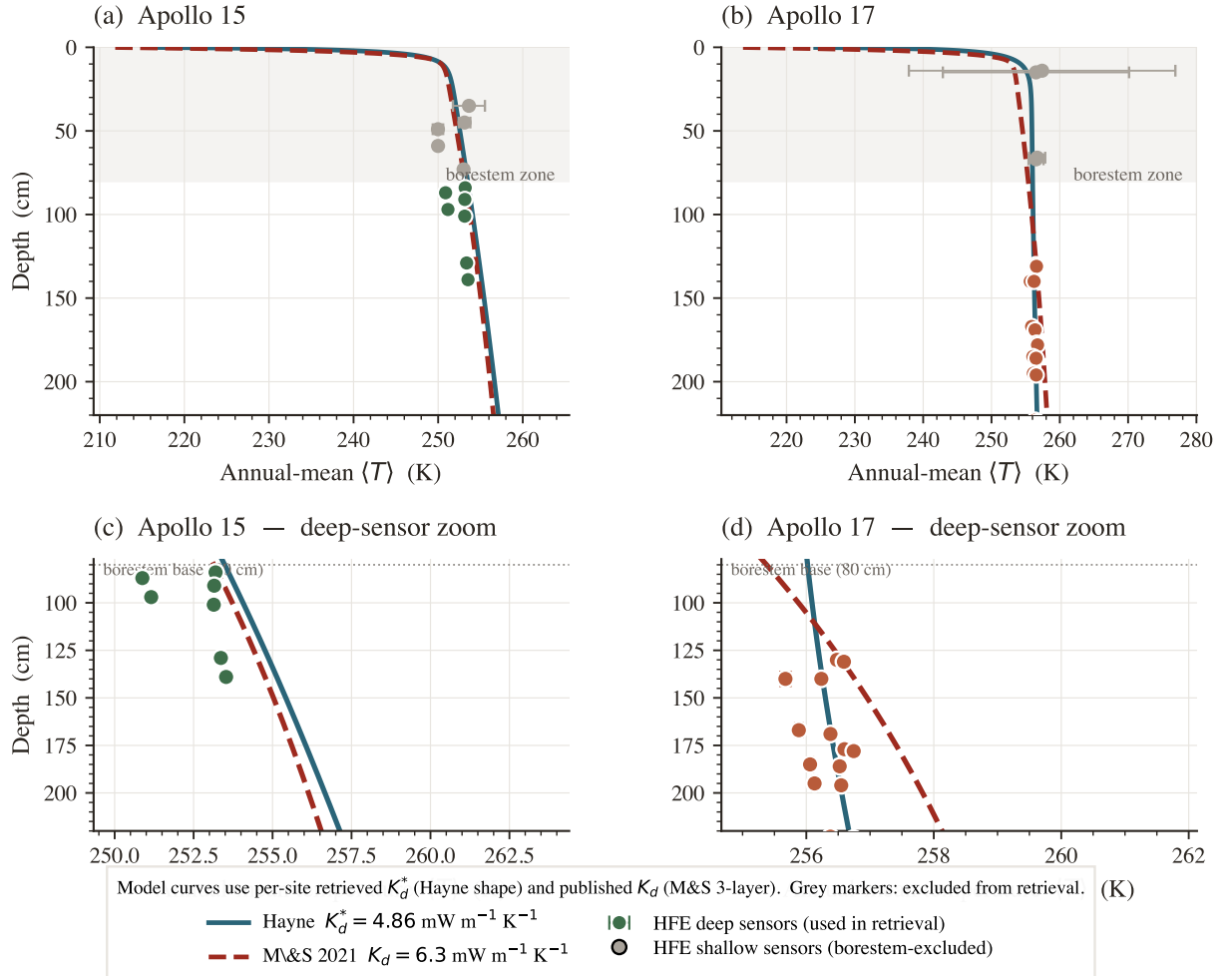
Figure 11. Annual-mean T(z) : Hayne with per-site K_d^* vs. Martínez and Siegler (2021) fixed K_d^{\text{disc}} = 6.3 . Solid teal: Hayne et al. (2017) at retrieved K_d^* . Dashed red: M&S 2021. Coloured markers: HFE deep sensors (used in retrieval); grey markers: borestem-affected shallow sensors (excluded).
