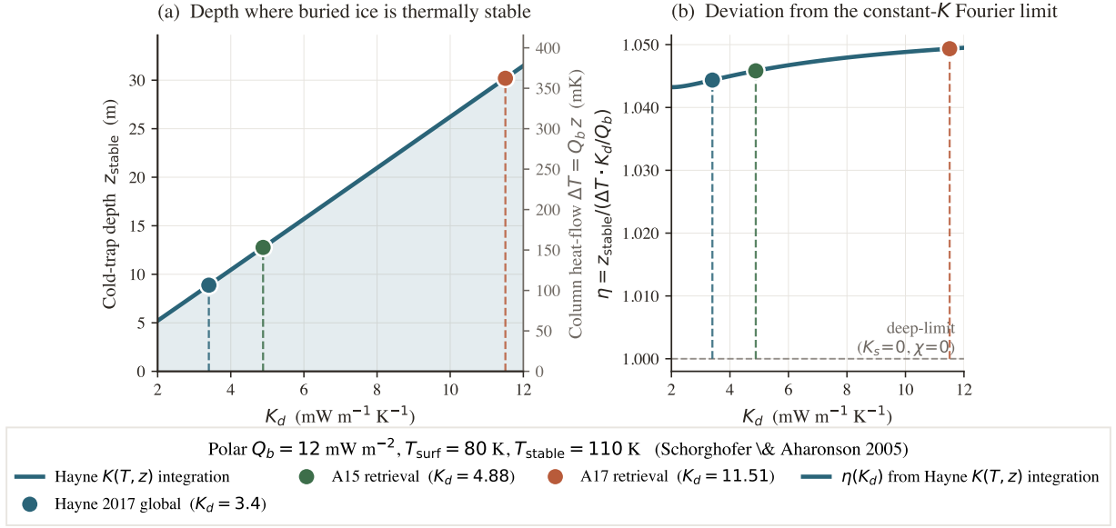
Figure 10. Polar cold-trap depth vs. K_d (Schorghofer-2005-style estimate at T_{\text{surf}} = 80 \text{ K} , Q_b = 12 \text{ mW/m}^2 ). (a) z_{\text{stable}} from forward-integrating dT/dz = Q_b/K(T, z) through the Hayne profile until T = T_{\text{stable}} = 110 \text{ K} ; right axis recasts the same depth as the column heat-flow drop \Delta T = Q_b z . (b) Ratio \eta = z_{\text{stable}}/[(\Delta T) K_d/Q_b] relative to the constant- K Fourier limit; \eta \approx 1.04 – 1.05 quantifies the shallow- K_s + radiative-term correction.
