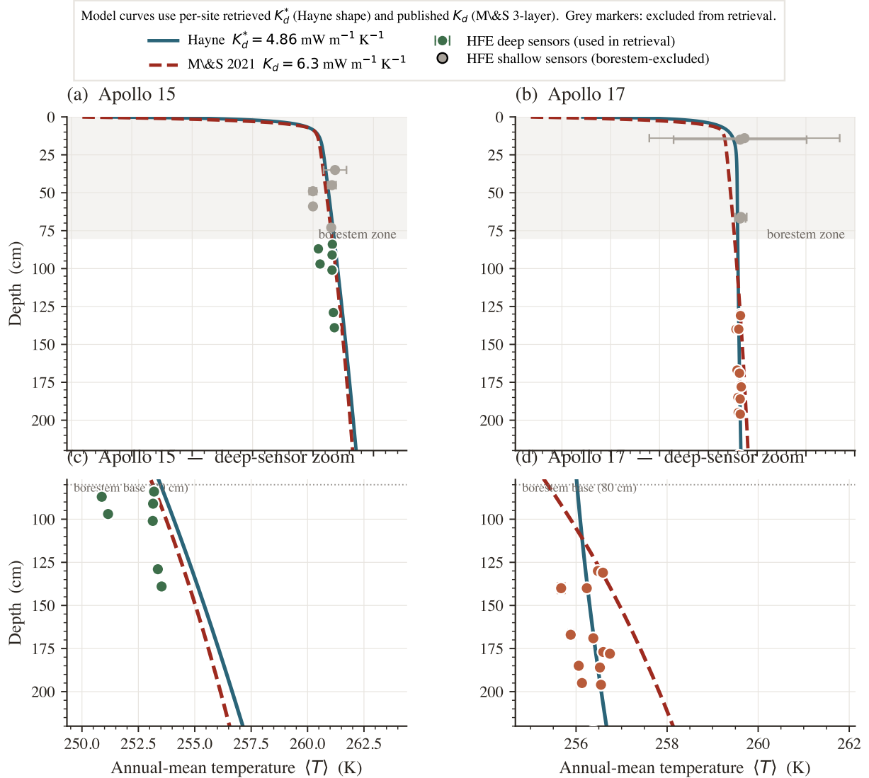
Figure 11. Annual-mean T(z) : Hayne with per-site K_d^* vs. Martínez and Siegler (2021) fixed K_d^{\text{disc}} = 6.3 . Solid teal: Hayne et al. (2017) at retrieved K_d^* . Dashed red: M&S 2021. Coloured markers: HFE deep sensors (used in retrieval); grey markers: borestem-affected shallow sensors (excluded).
