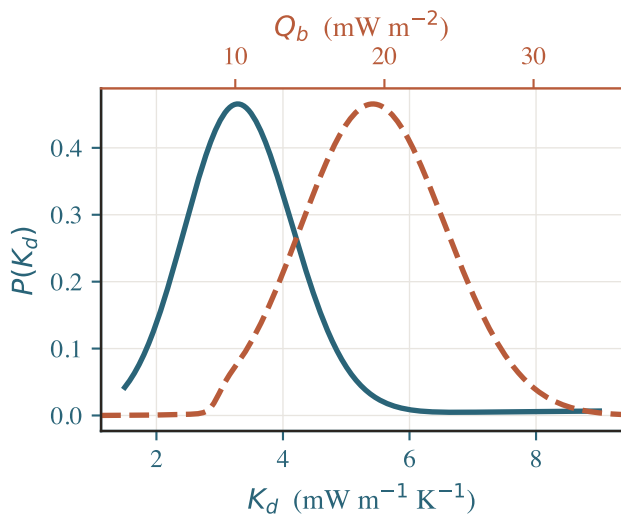
(c) A15 marginal posteriors
