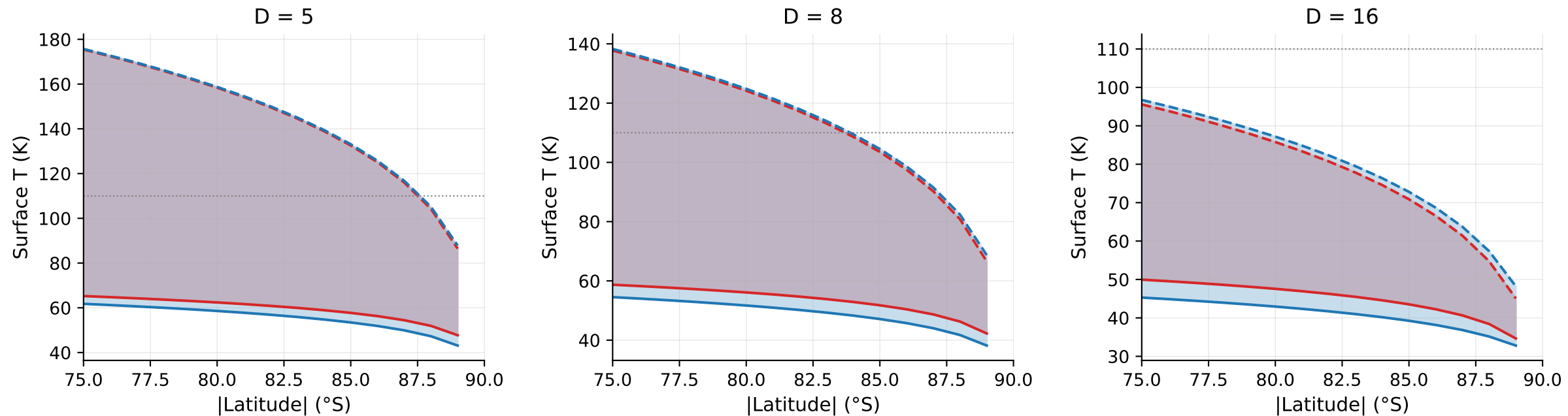
Crater floor T_{\min} / T_{\max} — Fig 8 of Martinez & Siegler (2021)
