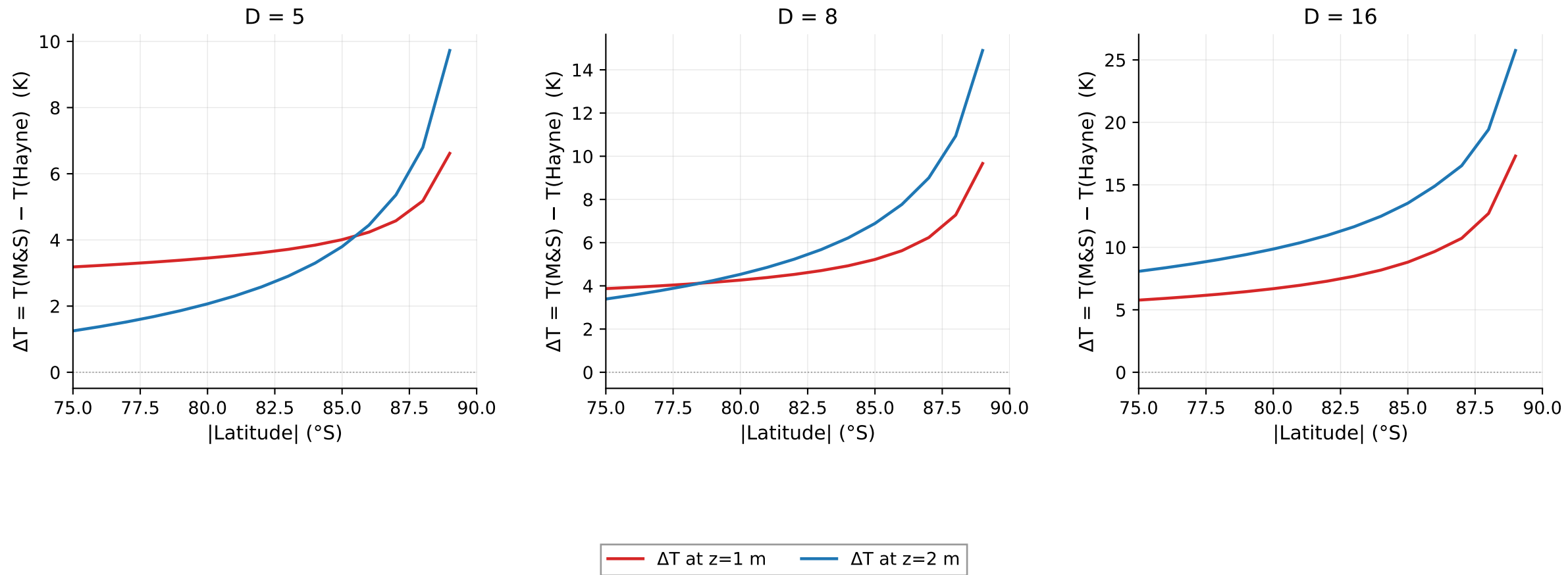
Crater \Delta T (M&S – Hayne) at 1m & 2m — Fig 9 of Martinez & Siegler (2021)
