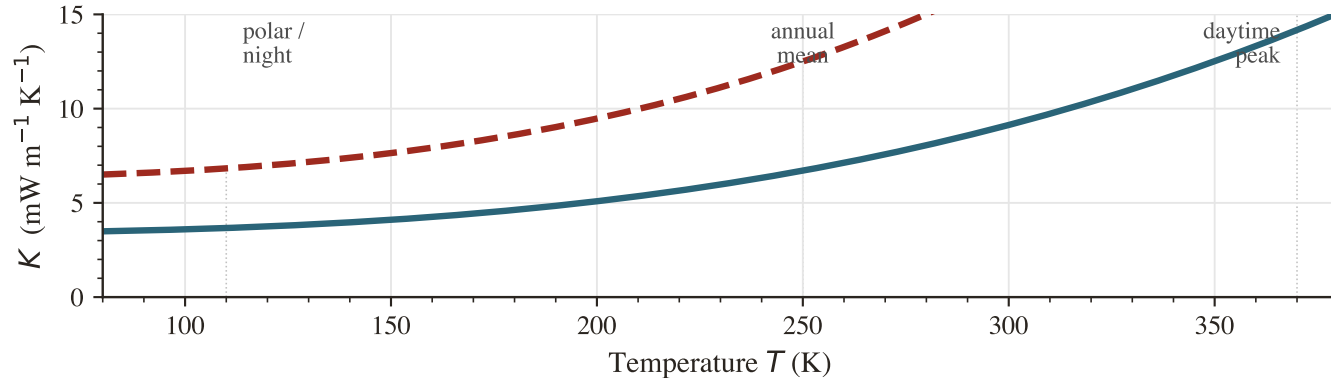
(c) K(T) at z = 30 \text{ cm} (deep limit; radiative multiplier dominates)
