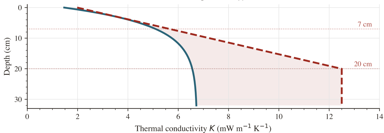
(b) K(z) at T = 250 \text{ K} (with radiative multiplier 1 + \chi(T/T_{\text{ref}})^3 )
