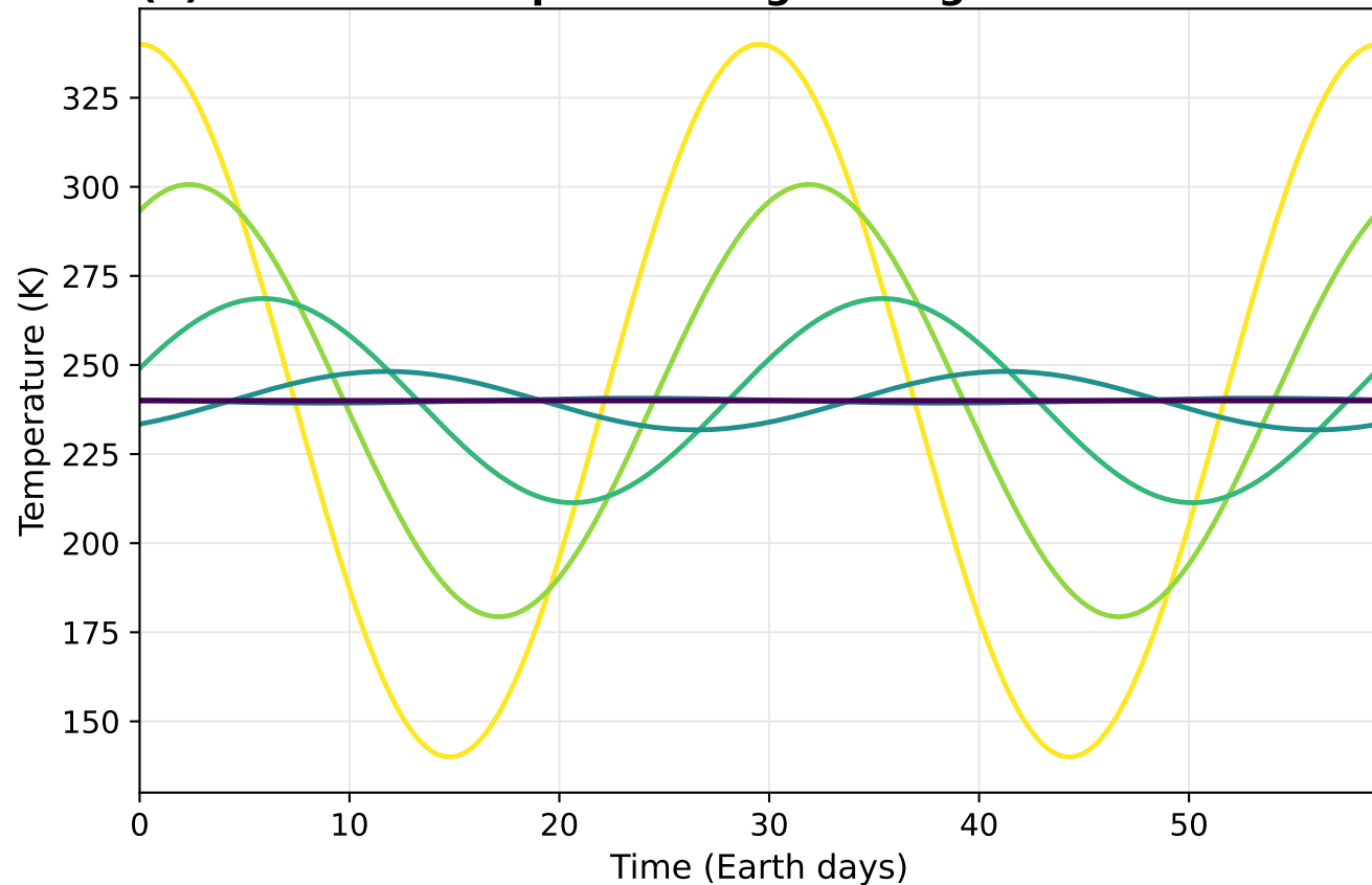
(a) Diurnal wave penetrating the regolith
