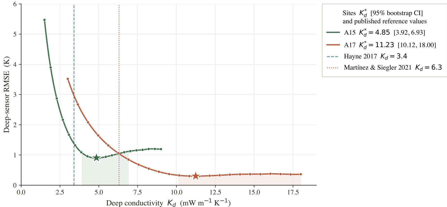
Per-site K_d retrieval under the Hayne 2017 functional form
