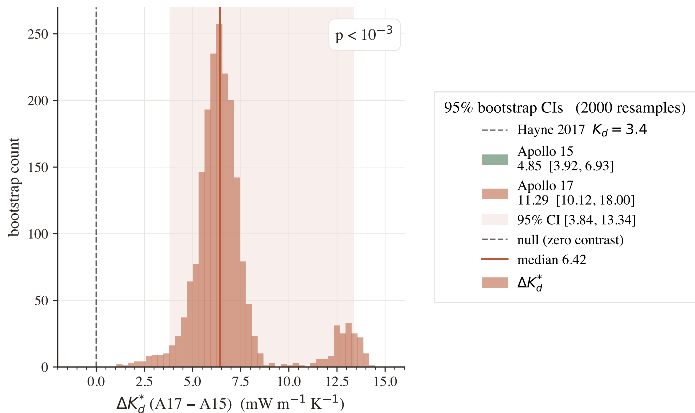
(b) Inter-site contrast distribution
