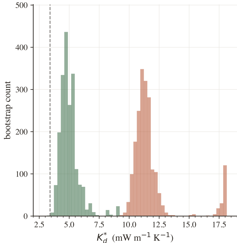
(a) Per-site bootstrap distributions
