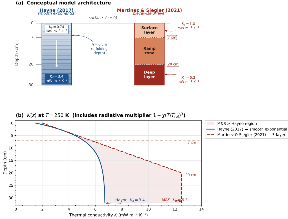
Figure 1. Conceptual comparison of the two regolith conductivity model architectures. (a) Physical layer structure: the Hayne et al. (2017) profile (blue) transitions continuously from a surface value K_s = 0.74 \text{ mW m}^{-1} \text{ K}^{-1} to a deep value K_d = 3.4 \text{ mW m}^{-1} \text{ K}^{-1} via an exponential with H = 6 \text{ cm} ; the Martínez and Siegler (2021) 3-layer profile (red) has a uniform surface layer ( K_s = 1.0 \text{ mW m}^{-1} \text{ K}^{-1} , 0–7 cm), a linear ramp zone (7–20 cm), and a uniform deep layer ( K_d = 6.3 \text{ mW m}^{-1} \text{ K}^{-1} , below 20 cm). (b) The corresponding K(z) profiles evaluated at T = 250 \text{ K} including the radiative multiplier 1 + \chi(T/T_{\text{ref}})^3 ; the shaded region is where the Martínez and Siegler (2021) conductivity exceeds the Hayne et al. (2017) value. The factor-of- \sim 2 difference in K_d is the dominant control on the deep-gradient discrepancy in Table 1.
