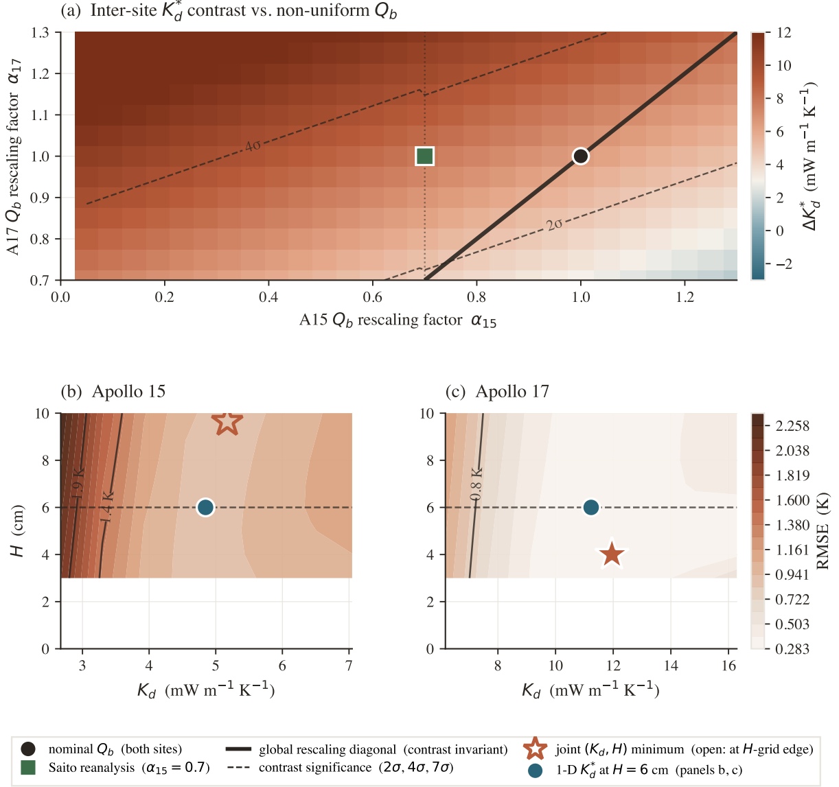
Figure 8. Robustness of the per-site K_d^* contrast. (a) Contrast \Delta K_d^* as a function of per-site Q_b rescaling factors \alpha_{15}, \alpha_{17} . Solid diagonal: global rescaling (contrast invariant); dashed contours: bootstrap- \sigma significance; black circle: nominal Q_b ; green square: Saito et al. (2007) A15 reanalysis. (b),(c) Joint (K_d, H) RMSE surface at each site; the coral star marks the joint RMSE minimum and the teal circle the 1-parameter retrieval at H = 6 cm. The RMSE surface is extremely flat in H — it varies by < 0.02 K across the swept H = 3 – 10 cm range — so H is effectively unconstrained and the joint minimum lies on the H -grid edge at both sites (open star). The retrieved K_d is nonetheless stable: the joint minimum and the 1-D retrieval agree in K_d to within the 0.5 K RMSE contour, confirming that K_d , not H , is the identified parameter.
