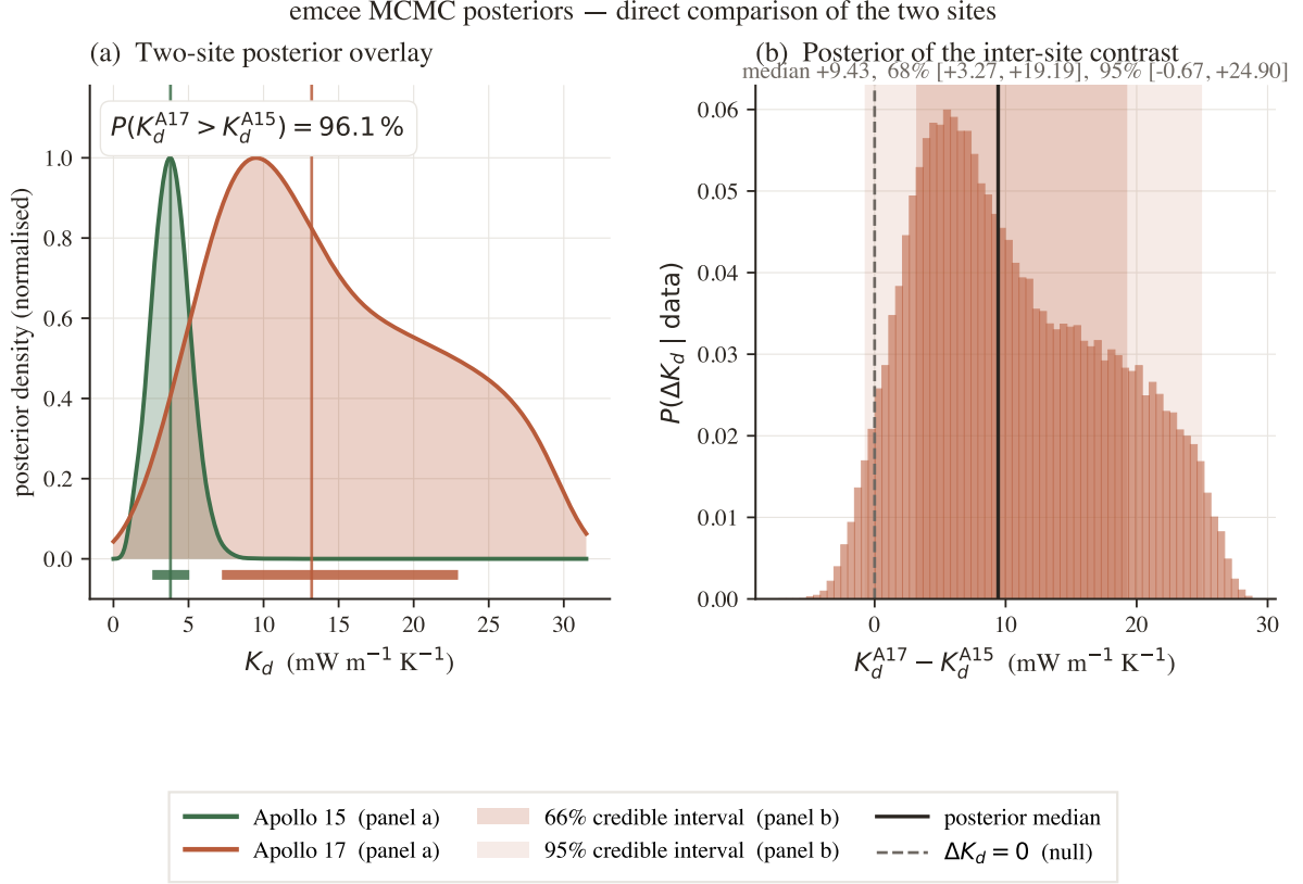
Figure 5.3. Direct two-site posterior comparison and contrast distribution. (a) Apollo 15 (teal) and Apollo 17 (coral) marginal P(K_d | \text{data}) overlaid as Gaussian-KDE estimates with median lines and 16–84 percentile bars at the foot of each curve. The annotated probability P(K_d^{A17} > K_d^{A15}) is the fraction of paired posterior draws for which the A17 sample exceeds the A15 sample, i.e. a distribution-level statement of how strongly the data discriminate the two sites. (b) Posterior of the inter-site contrast \Delta K_d \equiv K_d^{A17} - K_d^{A15} with 66% (darker) and 95% (lighter) credible intervals shaded; the dashed line at \Delta K_d = 0 marks the null hypothesis of a uniform deep conductivity. This is the Bayesian counterpart of the bootstrap contrast shown in the main letter.
