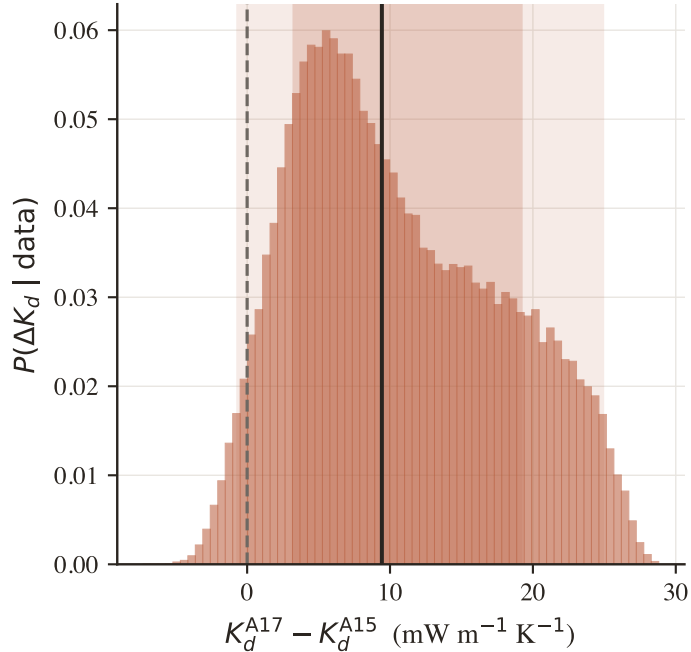
(b) Posterior of the inter-site contrast median +9.43, 68% [+3.27, +19.19], 95% [-0.67, +24.90]
