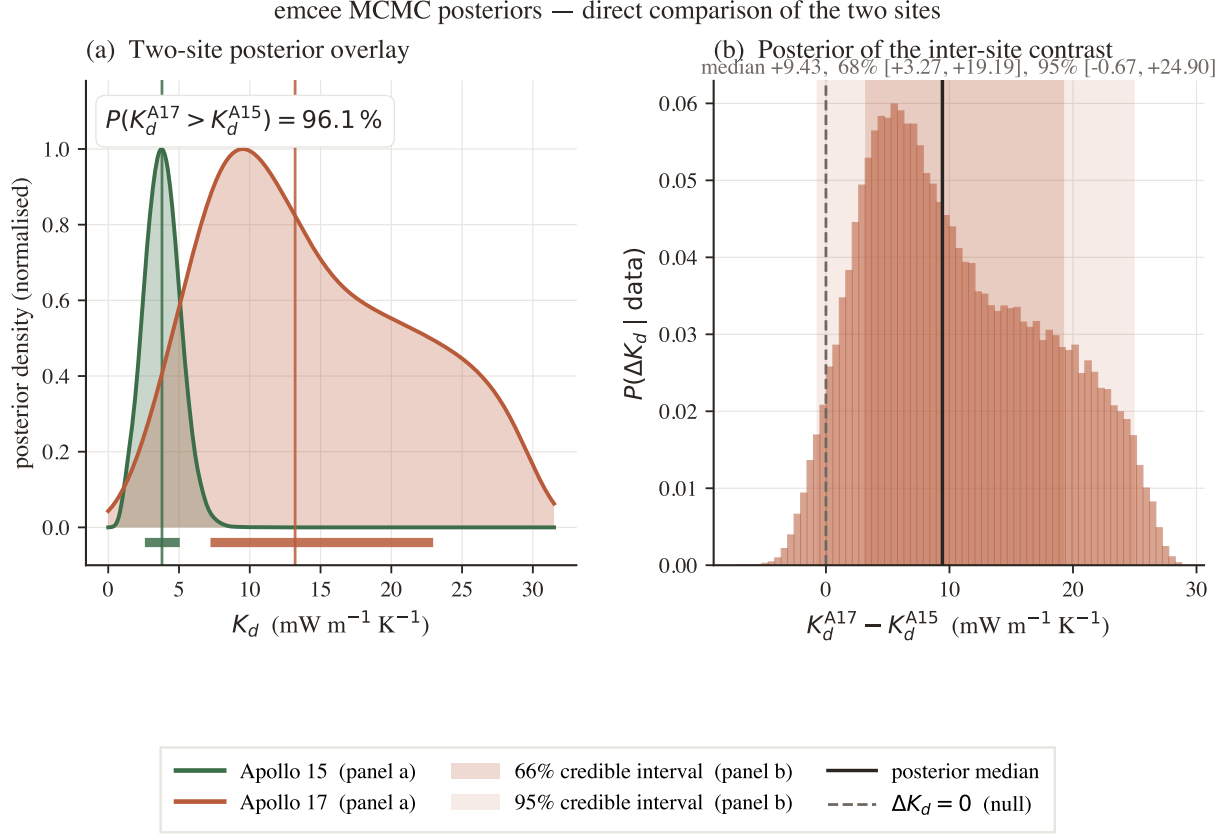
Figure 9. Direct two-site comparison of the MCMC posteriors. (a) The Apollo 15 (teal) and Apollo 17 (coral) marginal P(K_d | \text{data}) are overlaid on the same axes; filled curves are Gaussian-KDE estimates of the posterior, vertical lines mark medians, and the short bars at the foot of each curve span the 16–84 percentile range. The annotated probability is computed by drawing paired samples from the two marginals (the two sites’ data are independent), and quantifies how strongly the data discriminate K_d^{A17} from K_d^{A15} . (b) Posterior distribution of the inter-site contrast \Delta K_d \equiv K_d^{A17} - K_d^{A15} , formed from the same paired draws. The 66% (darker) and 95% (lighter) credible intervals are shaded; the dashed line at \Delta K_d = 0 shows the null hypothesis of a uniform deep conductivity. The bulk of the posterior mass lies well above zero, providing a clean distribution-level statement of the regional heterogeneity finding that complements the bootstrap-based contrast in Fig. 5.
