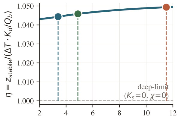
(b) Deviation from the constant- K Fourier limit
