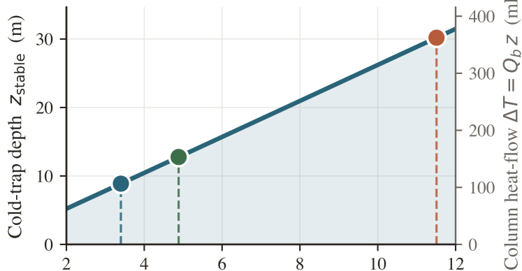
(a) Depth where buried ice is thermally stable
