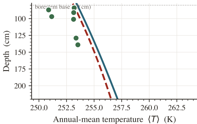
(c) Apollo 15 — deep-sensor zoom
