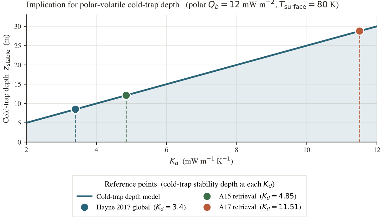
Figure 10. Implication for polar volatile cold-trap depth. Indicative cold-trap depth z_{\text{stable}} at which buried water ice is thermally stable on geological timescales (a Schorghofer and Aharonson 2005-style estimate at fixed polar surface temperature and basal heat flux), as a function of K_d . The factor-of- \sim 3 change in K_d between the global value of Hayne et al. (2017) and the A17 retrieval translates into a factor-of- \sim 3 change in z_{\text{stable}} .
