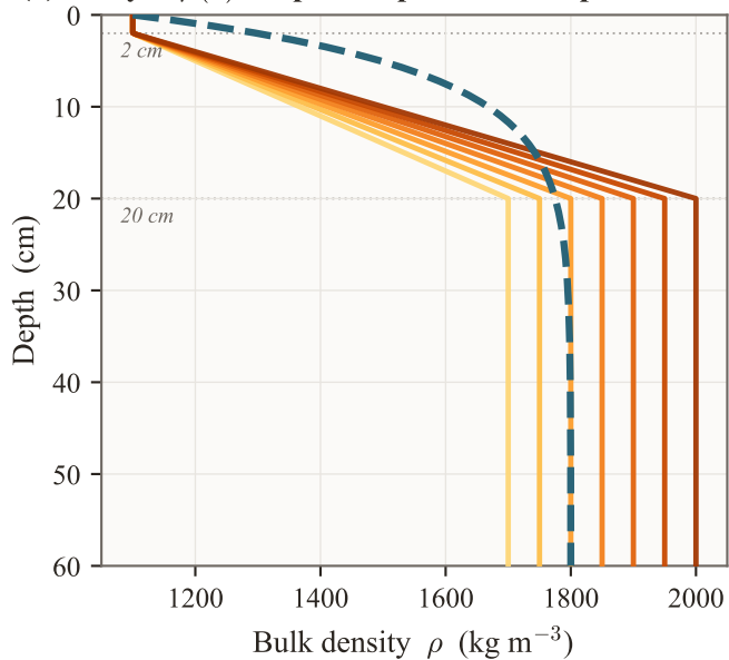
(a) 3-layer \rho(z) shapes swept over the Apollo-core range
