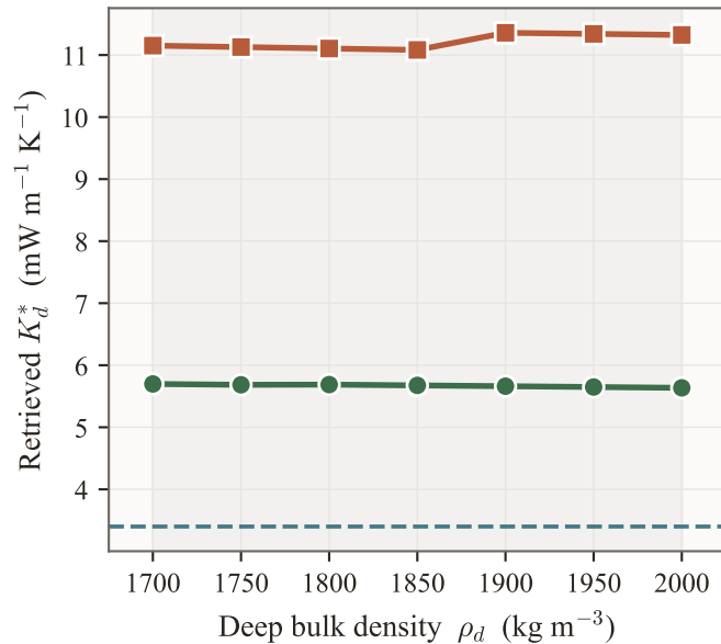
(b) K_d^* response across the same range
