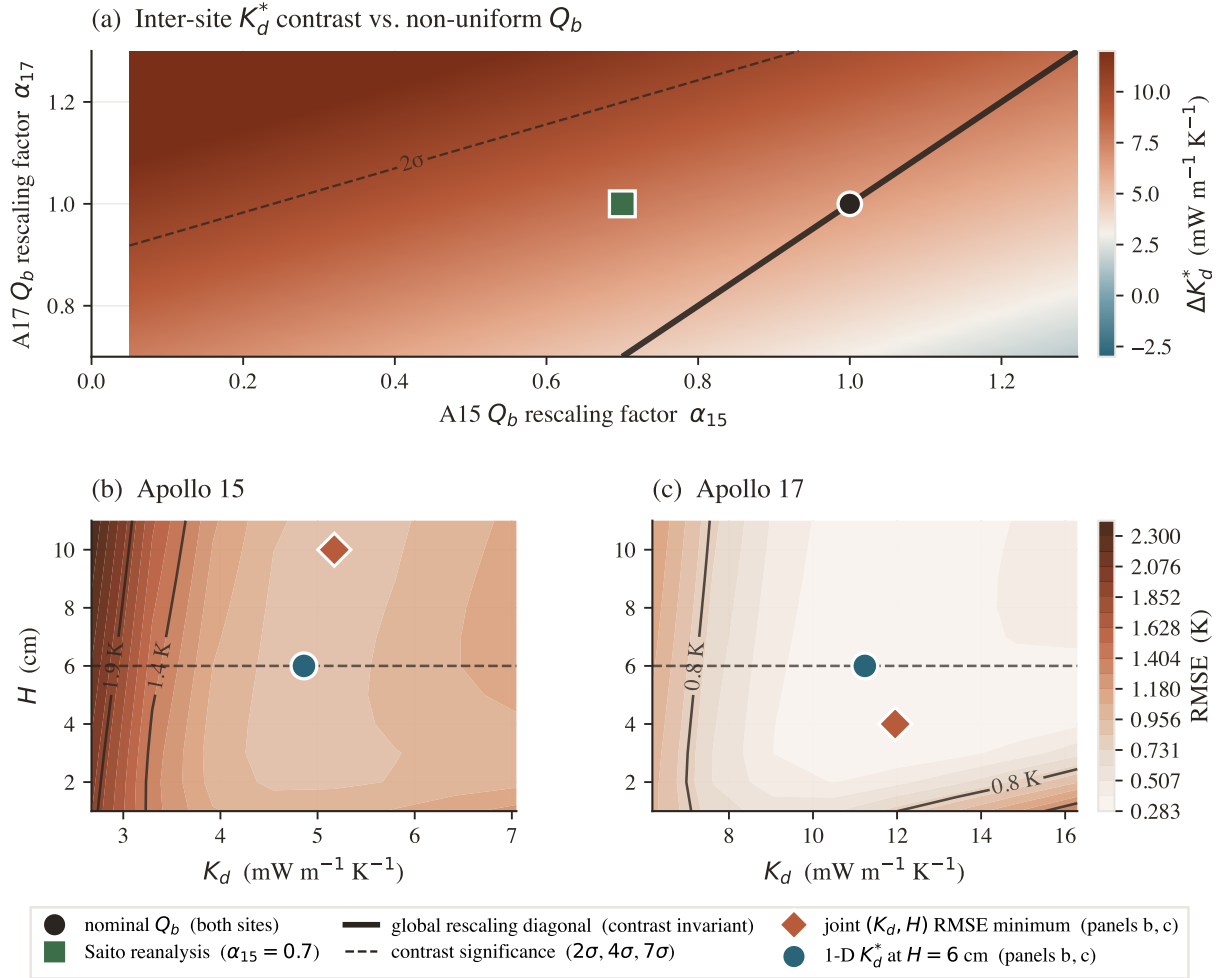
Figure 8. Robustness of the per-site K_d^* contrast. (a) Contrast \Delta K_d^* as a function of per-site Q_b rescaling factors \alpha_{15}, \alpha_{17} . Solid diagonal: global rescaling (contrast invariant); dashed contours: bootstrap- \sigma significance; black circle: nominal Q_b ; green square: Saito et al. (2007) A15 reanalysis. (b),(c) Joint (K_d, H) RMSE surface at each site over the swept H = 1\text{--}11 cm range; the coral diamond marks the joint RMSE minimum and the teal circle the 1-parameter retrieval at H = 6 cm. The RMSE surface is extremely flat in H — it varies by < 0.02 K across H = 3\text{--}11 cm — so H is effectively unconstrained, with shallow interior minima at H \approx 10 cm (A15) and 4 cm (A17). The retrieved K_d is nonetheless stable: the joint minimum and the 1-D retrieval agree in K_d to within the 0.5 K RMSE contour, confirming that K_d , not H , is the identified parameter.
