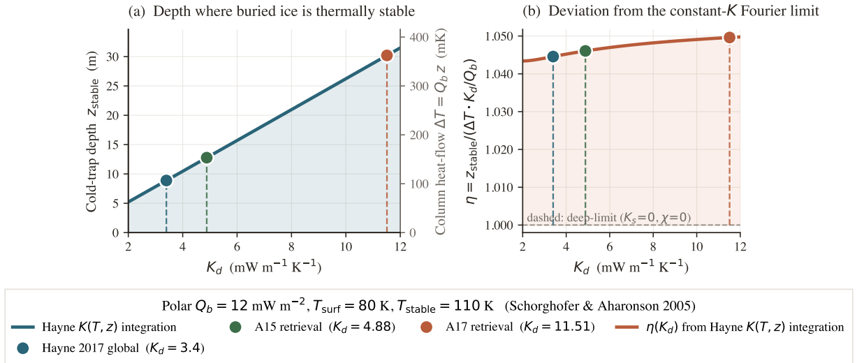
Figure 11. Polar cold-trap depth vs. K_d (Schorghofer-2005-style estimate at T_{\text{surf}} = 80\text{ K} , Q_b = 12\text{ mW}/\text{m}^2 ). (a) z_{\text{stable}} from RK4 forward-integration of dT/dz = Q_b/K(T, z) through the Hayne K(T, z) profile until T = T_{\text{stable}} = 110\text{ K} ; the right axis recasts the same depth as the column heat-flow drop \Delta T = Q_b z . The curve is close to linear because the Q_b/K_d term dominates. (b) Ratio \eta = z_{\text{stable}} / [(\Delta T) K_d / Q_b] relative to the constant- K Fourier limit; \eta \approx 1.04\text{--}1.05 resolves the mild ( \sim 5\% ) departure from linearity from the shallow- K_s layer and the radiative term.
