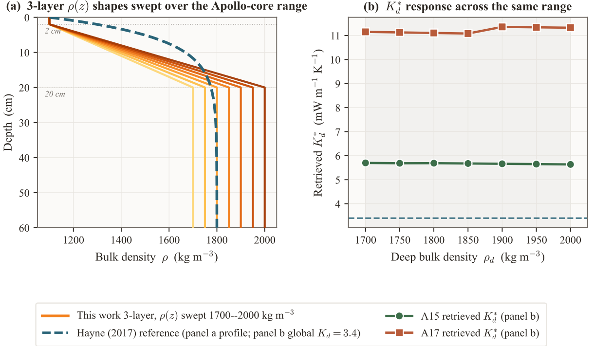
Figure 2. The this-work discrete three-layer conductivity model and its sensitivity to the deep bulk density \rho_d . (a) Family of \rho(z) profiles obtained by sweeping \rho_d across the 1700–2000 \text{kg m}^{-3} range spanned by the Apollo regolith cores (Mitchell et al., 1973; Carrier et al., 1991); the Hayne et al. (2017) smooth-exponential profile is shown for reference. (b) Retrieved deep conductivity K_d^* at each site as a function of the assumed \rho_d (per-site values from §3.5, foreshadowed here). The Apollo 15 and 17 retrievals are flat in \rho_d to within 1.1% and 2.4% across the full range, indicating that the per-site K_d^* is essentially independent of the precise \rho_d chosen so long as it lies within the observed Apollo-core range; both sit well above the Hayne et al. (2017) global K_d = 3.4 \text{ mW m}^{-1} \text{ K}^{-1} (dashed teal).
