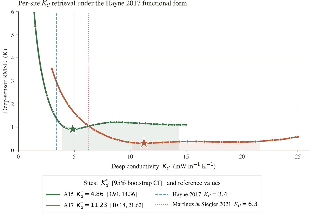
Figure 5. Per-site K_d retrieval under the Hayne et al. (2017) functional form. Deep-sensor RMSE vs K_d , with the other Hayne et al. (2017) parameters held at their published values. Filled markers: swept grid; solid curve: parabolic refinement near the minimum; shaded band: bootstrap 95% CI. Dashed vertical: Hayne et al. (2017) global K_d = 3.4 ; dotted: Martínez and Siegler (2021) K_d = 6.3 .
