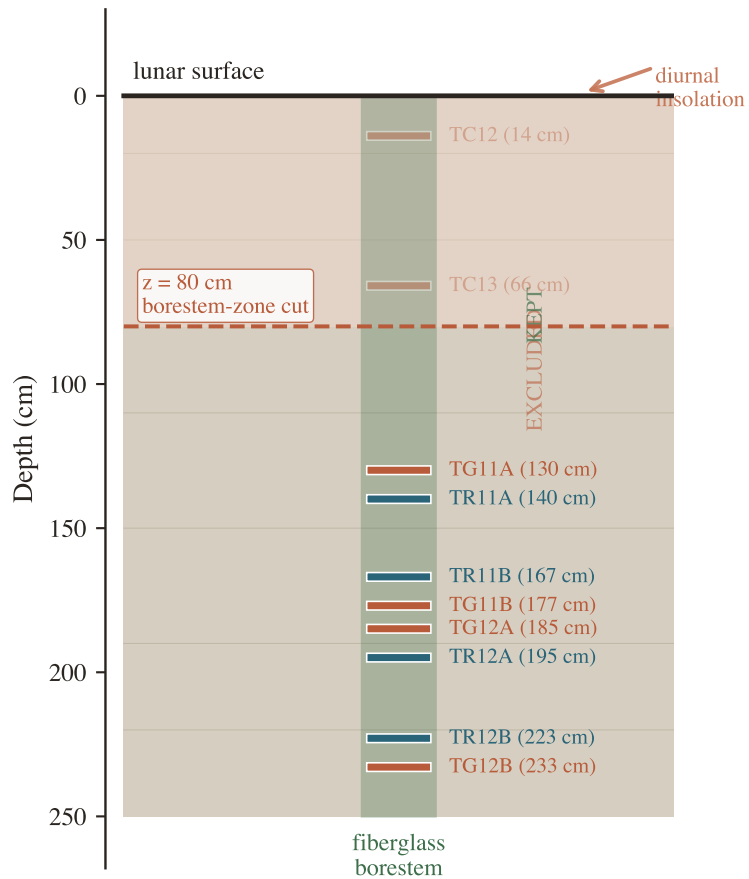
(a) HFE probe in regolith column
