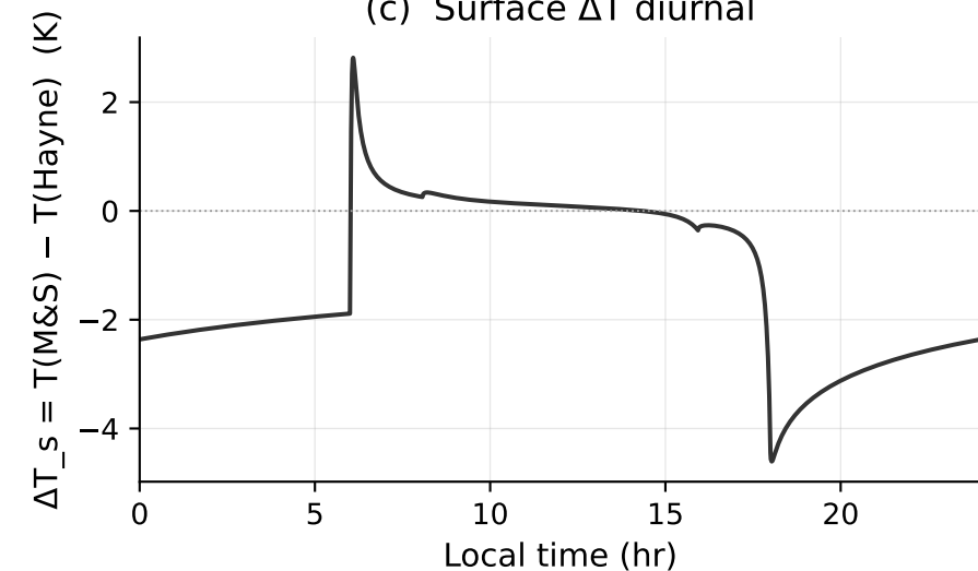
(c) Surface \Delta T diurnal
