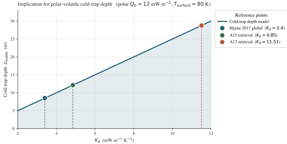
Figure 9.4. Implication for polar volatile cold-trap depth. Indicative cold-trap depth z_{\text{stable}} at which buried water ice is thermally stable on geological timescales (a Schorghofer and Aharonson 2005-style estimate at fixed polar surface temperature and basal heat flux), as a function of K_d . The factor-of- \sim 3 change in K_d between the global value of Hayne et al. (2017) and the A17 retrieval translates into a factor-of- \sim 3 change in z_{\text{stable}} , illustrating that the regional heterogeneity in K_d reported here is large enough to matter for downstream volatile-stability budgets.
