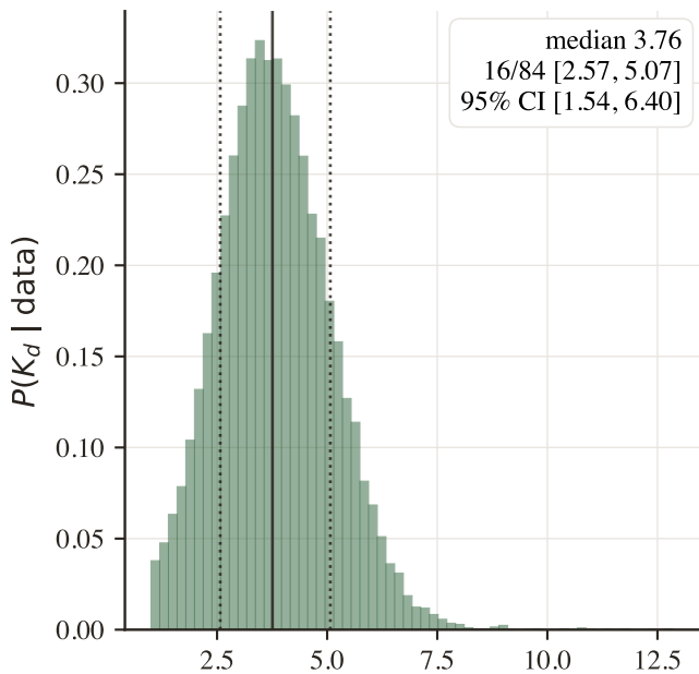
(c) Apollo 15 — marginal P(K_d)
