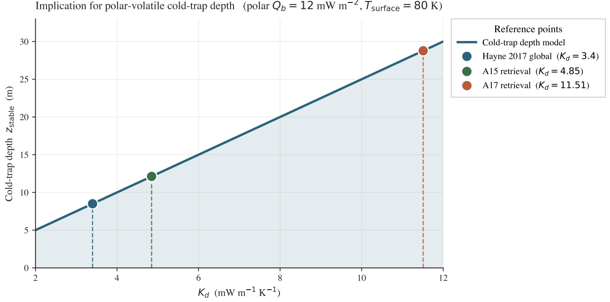
Figure 9. Implication for polar volatile cold-trap depth. Indicative cold-trap depth z_{\text{stable}} at which buried water ice is thermally stable on geological timescales (a Schorghofer and Aharonson 2005-style estimate at fixed polar surface temperature and basal heat flux), as a function of K_d . The factor-of- \sim 3 change in K_d between the global value of Hayne et al. (2017) and the A17 retrieval translates into a factor-of- \sim 3 change in z_{\text{stable}} .
