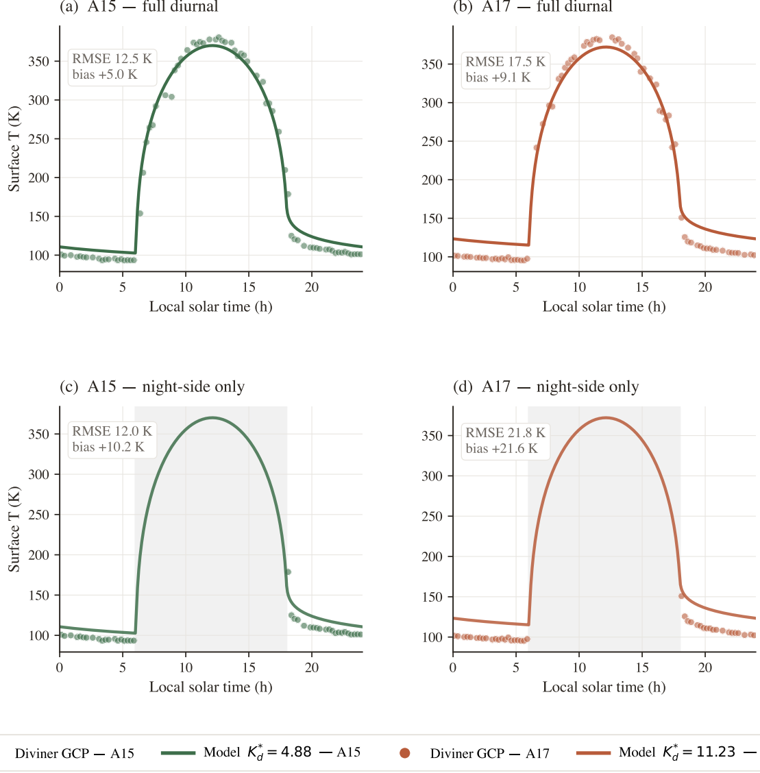
Figure 7. Surface-temperature closure against the Diviner Lunar Radiometer Global Cumulative Product (Williams et al., 2017). (a)–(b) Full diurnal cycle at A15 and A17: dots are Diviner brightness temperatures binned at 0.25-h LST resolution within \pm 0.5^\circ latitude and \pm 1^\circ longitude of each landing site; solid curves are the modelled surface temperature run with the per-site retrieved K_d^* . (c)–(d) Same comparison restricted to the night side (LST in [0, 6] \cup [18, 24] ; day-side shaded). The full-cycle warm-bias has a daytime anisothermal component plus a residual night-side offset most plausibly attributable to local-scale albedo / emissivity variations relative to the Vasavada et al. (2012) latitude-band averages we adopt. Neither component propagates to the deep K_d retrieval, which constrains the deep equilibrium gradient Q_b/K_d rather than the absolute surface temperature.
