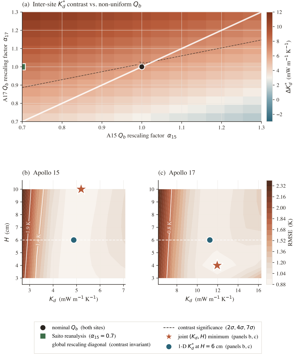
Figure 6. Robustness of the per-site K_d^* contrast. (a) Inter-site contrast \Delta K_d^* as a function of independent per-site rescaling factors \alpha_{15}, \alpha_{17} on the published basal heat fluxes; the white diagonal marks global rescaling, under which the contrast is exactly invariant. Dashed contours give the bootstrap-normalised significance ( \sigma ). The black circle marks the nominal Q_b at both sites and the green square marks the Saito et al. (2007) ; Nagihara et al. (2018) reanalysis at A15. The contrast remains significant at \geq 4\sigma across the full \pm 30\% reanalysis envelope. (b)–(c) Two-parameter joint fit of K_d and the e-folding depth H at each site; white contours are at the labelled RMSE values above the joint minimum. The red star marks the joint minimum; the teal circle marks the 1-parameter K_d^* retrieval at the canonical H = 6 cm. The two minima coincide to within the 0.5 K RMSE contour, indicating that K_d is the dominant identified lever and that the retrieval is not a degenerate trade-off with H .
