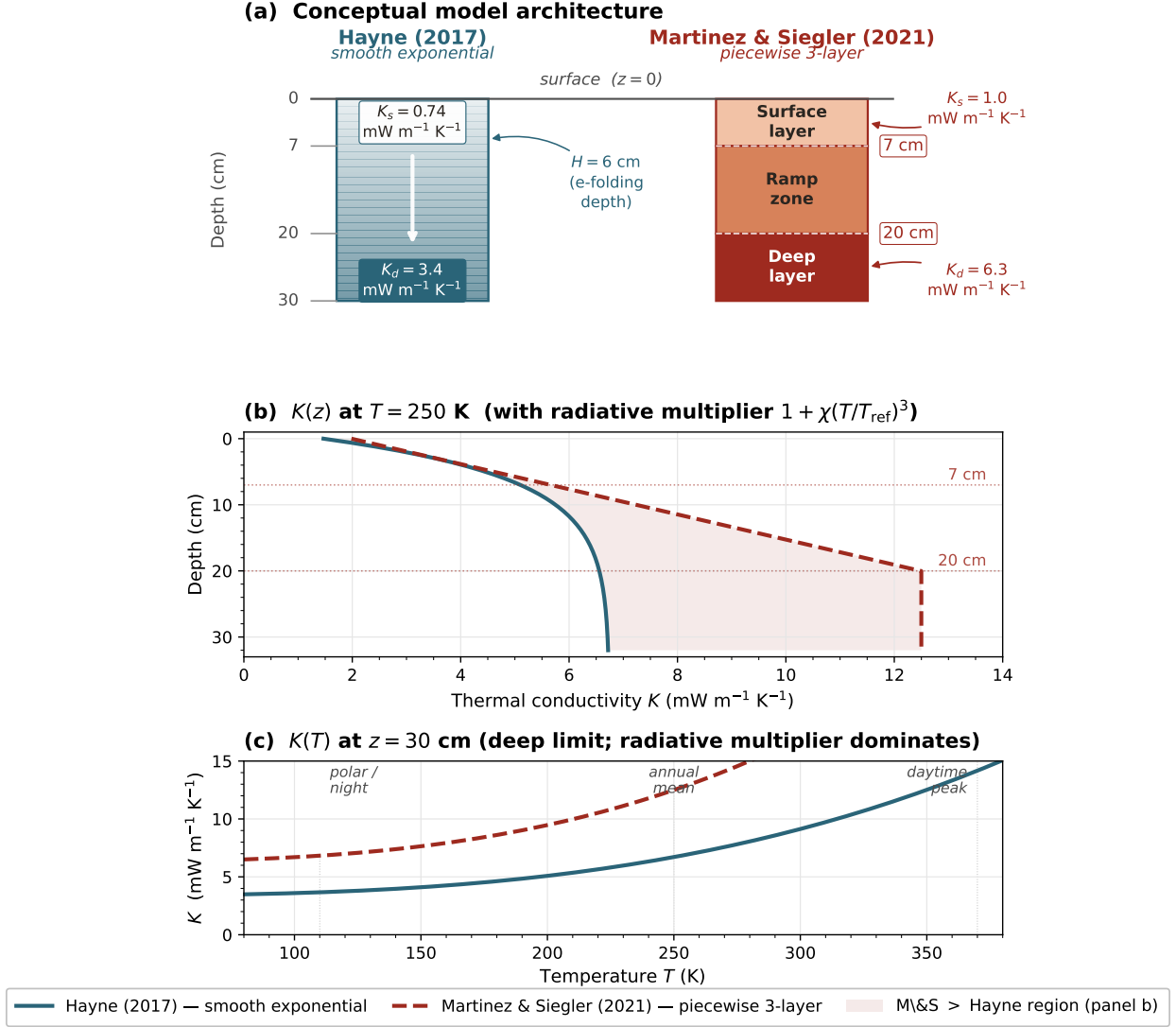
Figure 1. Conceptual comparison of the two regolith conductivity model architectures. (a) Physical layer structure: the Hayne et al. (2017) profile (blue) transitions continuously from a surface value K_s = 0.74 \text{ mW m}^{-1} \text{ K}^{-1} to a deep value K_d = 3.4 \text{ mW m}^{-1} \text{ K}^{-1} via an exponential with H = 6 \text{ cm} ; the Martínez and Siegler (2021) 3-layer profile (red) has a uniform surface layer ( K_s = 1.0 \text{ mW m}^{-1} \text{ K}^{-1} , 0–7 cm), a linear ramp zone (7–20 cm), and a uniform deep layer ( K_d = 6.3 \text{ mW m}^{-1} \text{ K}^{-1} , below 20 cm). (b) The corresponding K(z) profiles evaluated at T = 250 \text{ K} including the radiative multiplier 1 + \chi(T/T_{\text{ref}})^3 ; the shaded region is where the Martínez and Siegler (2021) conductivity exceeds the Hayne et al. (2017) value. The factor-of- \sim 2 difference in K_d is the dominant control on the deep-gradient discrepancy in Table 1.
