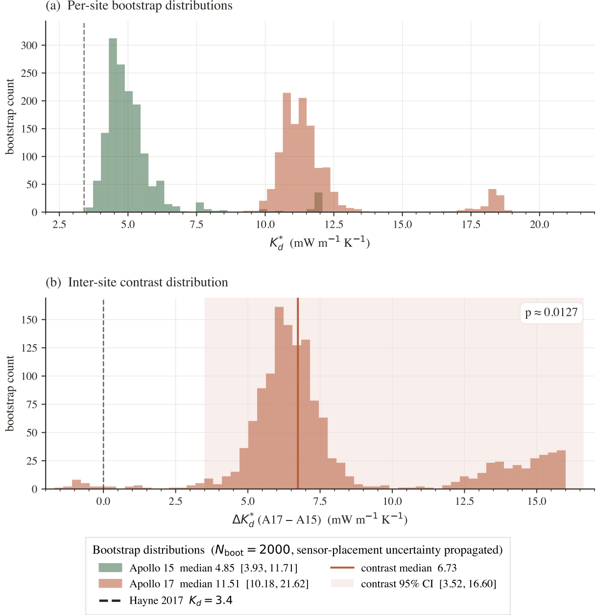
Figure 5. Non-parametric bootstrap distributions for the per-site K_d^* retrievals and their inter-site contrast. (a) Bootstrap histograms of K_d^* from N_{\text{boot}} = 2000 resamples of the deep-sensor set at each site (with replacement and with the published \pm 2.5 cm sensor-placement uncertainty propagated). The 95% confidence intervals are listed in the legend. The vertical dashed line marks the published global value K_d = 3.4 \text{ mW}/(\text{m K}) . (b) Distribution of the inter-site contrast \Delta K_d^* = K_{d,A17}^* - K_{d,A15}^* , with the 95% bootstrap CI shaded. The distribution does not overlap zero, giving p \approx 0.013 for the null of inter-site equality.
