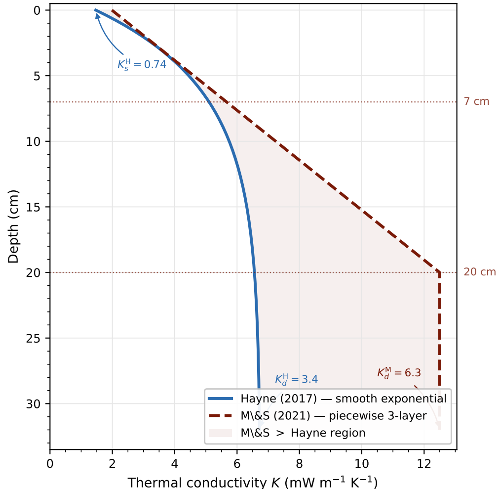
(b) K(z) at T = 250 K (including radiative term 1 + \chi(T/T_{\text{ref}})^3 )
