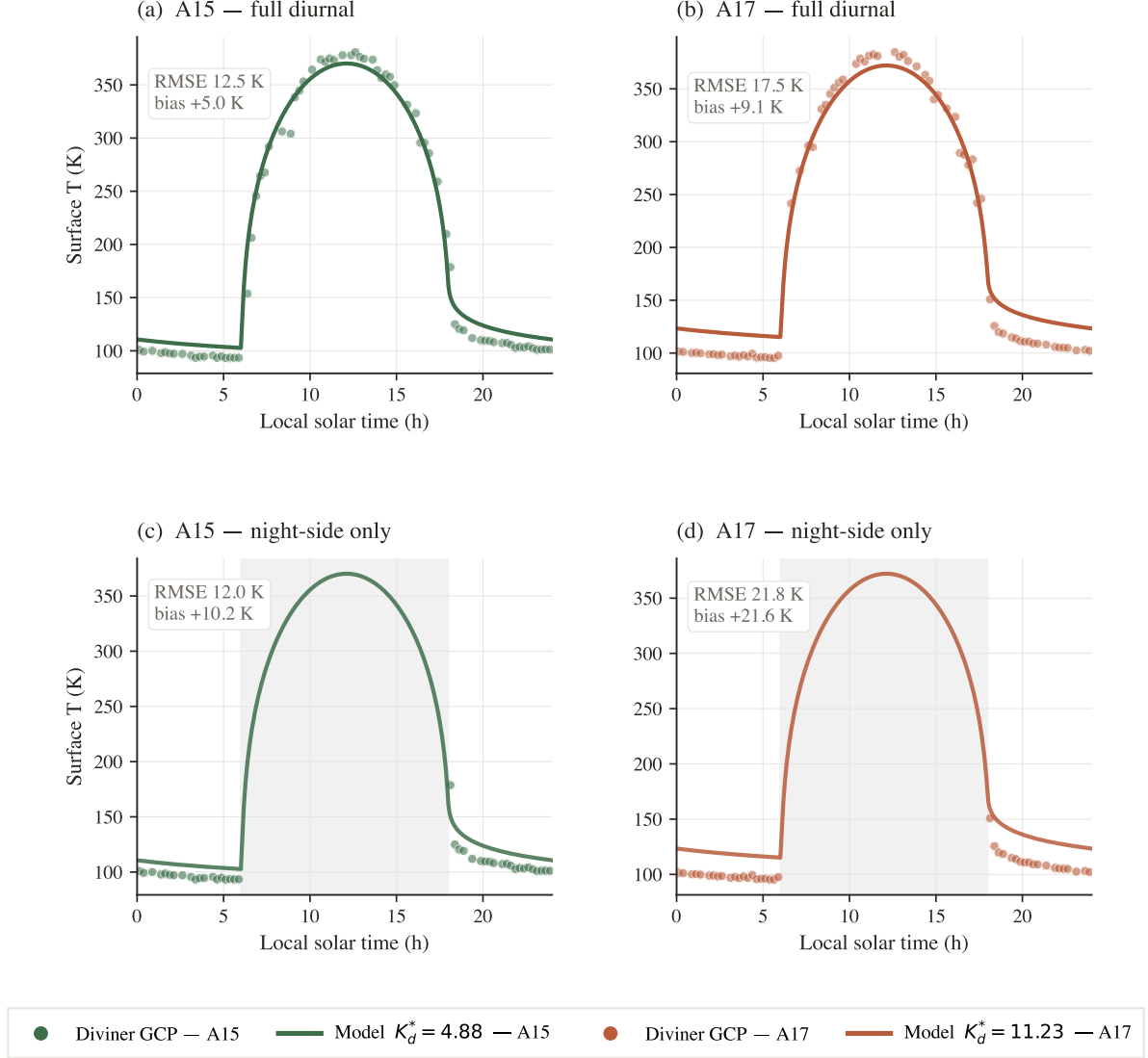
Figure 10.5. Surface-temperature closure against the Diviner GCP. (a)–(b) Full diurnal cycle at each site: dots are the Diviner brightness temperature binned at 0.25-h LST resolution within \pm 0.5^\circ latitude and \pm 1^\circ longitude of each landing site; solid curves are the modelled surface temperature run with the per-site retrieved K_d^* . (c)–(d) Night-side-only restriction (LST in [0, 6] \cup [18, 24] ; day-side shaded). The full-cycle bias has a daytime anisothermal component plus a residual night-side offset that is most plausibly caused by local-scale bolometric-albedo / emissivity variations. Neither component propagates into the deep K_d retrieval, which constrains the deep equilibrium gradient Q_b/K_d and not the absolute surface temperature.
