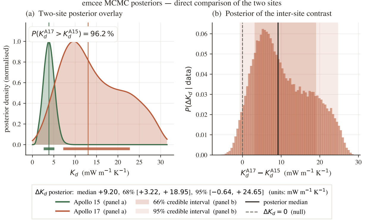
Figure 9. Direct two-site comparison of the MCMC posteriors. (a) The Apollo 15 (teal) and Apollo 17 (coral) marginal P(K_d | \text{data}) are overlaid on the same axes; filled curves are Gaussian-KDE estimates of the posterior, vertical lines mark medians, and the short bars at the foot of each curve span the 16–84 percentile range. The annotated probability is computed by drawing paired samples from the two marginals (the two sites’ data are independent), and quantifies how strongly the data discriminate K_d^{A17} from K_d^{A15} . (b) Posterior distribution of the inter-site contrast \Delta K_d \equiv K_d^{A17} - K_d^{A15} , formed from the same paired draws. The 66% (darker) and 95% (lighter) credible intervals are shaded; the dashed line at \Delta K_d = 0 shows the null hypothesis of a uniform deep conductivity. The bulk of the posterior mass lies well above zero, providing a clean distribution-level statement of the regional heterogeneity finding that complements the bootstrap-based contrast in Fig. 5.
