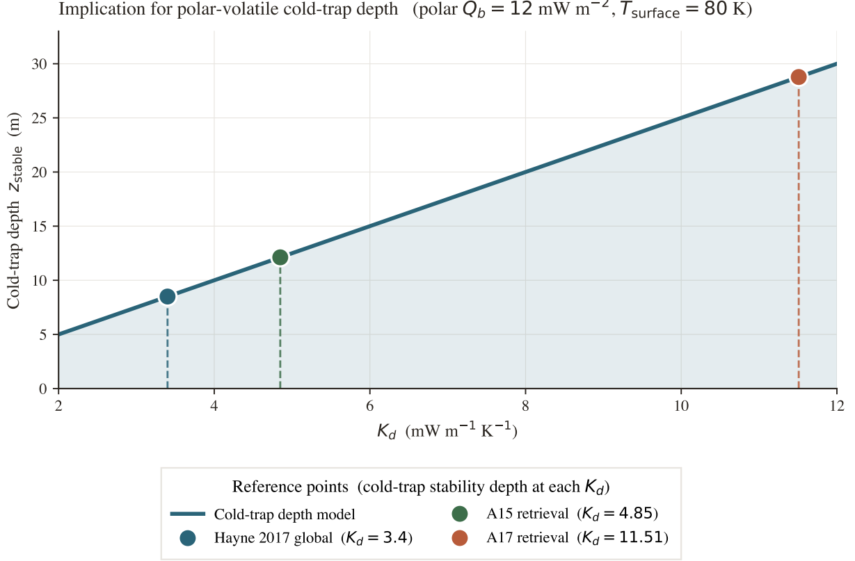
Figure 10. Implication for polar volatile cold-trap depth. Indicative cold-trap depth z_{\text{stable}} at which buried water ice is thermally stable on geological timescales (a Schorghofer and Aharonson 2005-style estimate at fixed polar surface temperature and basal heat flux), as a function of K_d . The factor-of- \sim 3 change in K_d between the global value of Hayne et al. (2017) and the A17 retrieval translates into a factor-of- \sim 3 change in z_{\text{stable}} .
