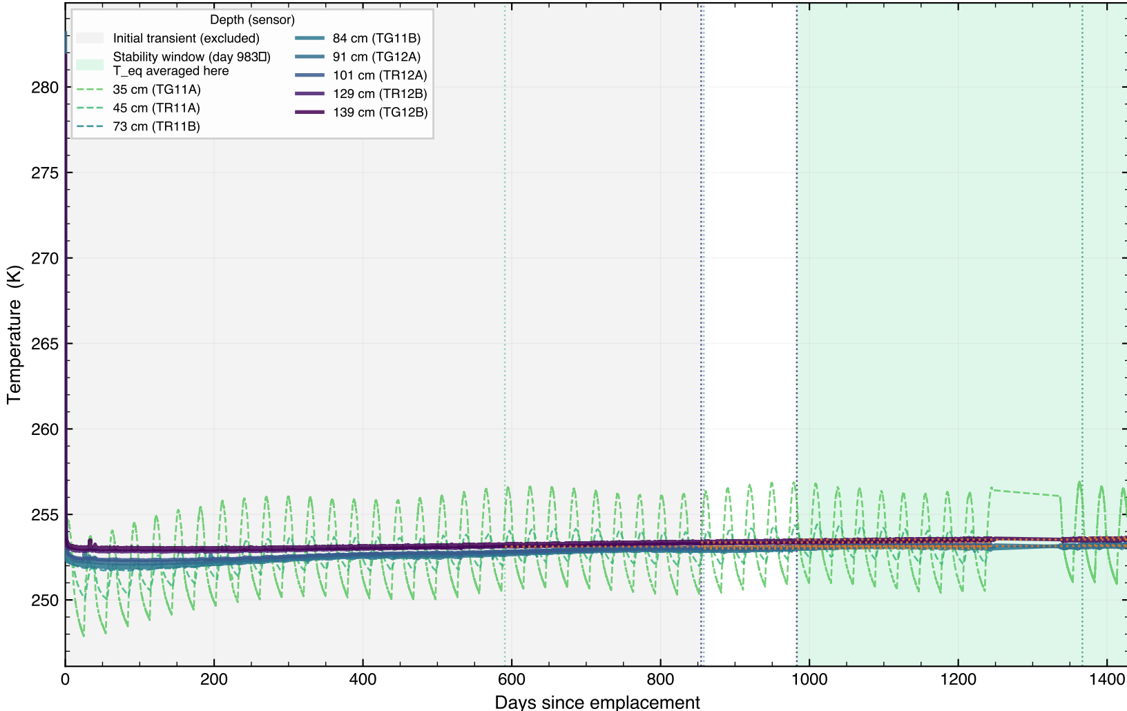
Apollo 15 — Probe 1 (Thermal Stability Analysis)
