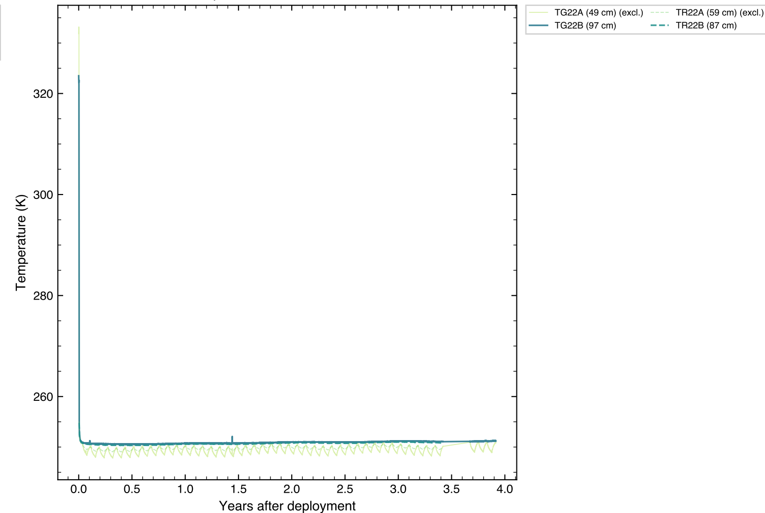
Apollo 15 HFE — Probe 2
