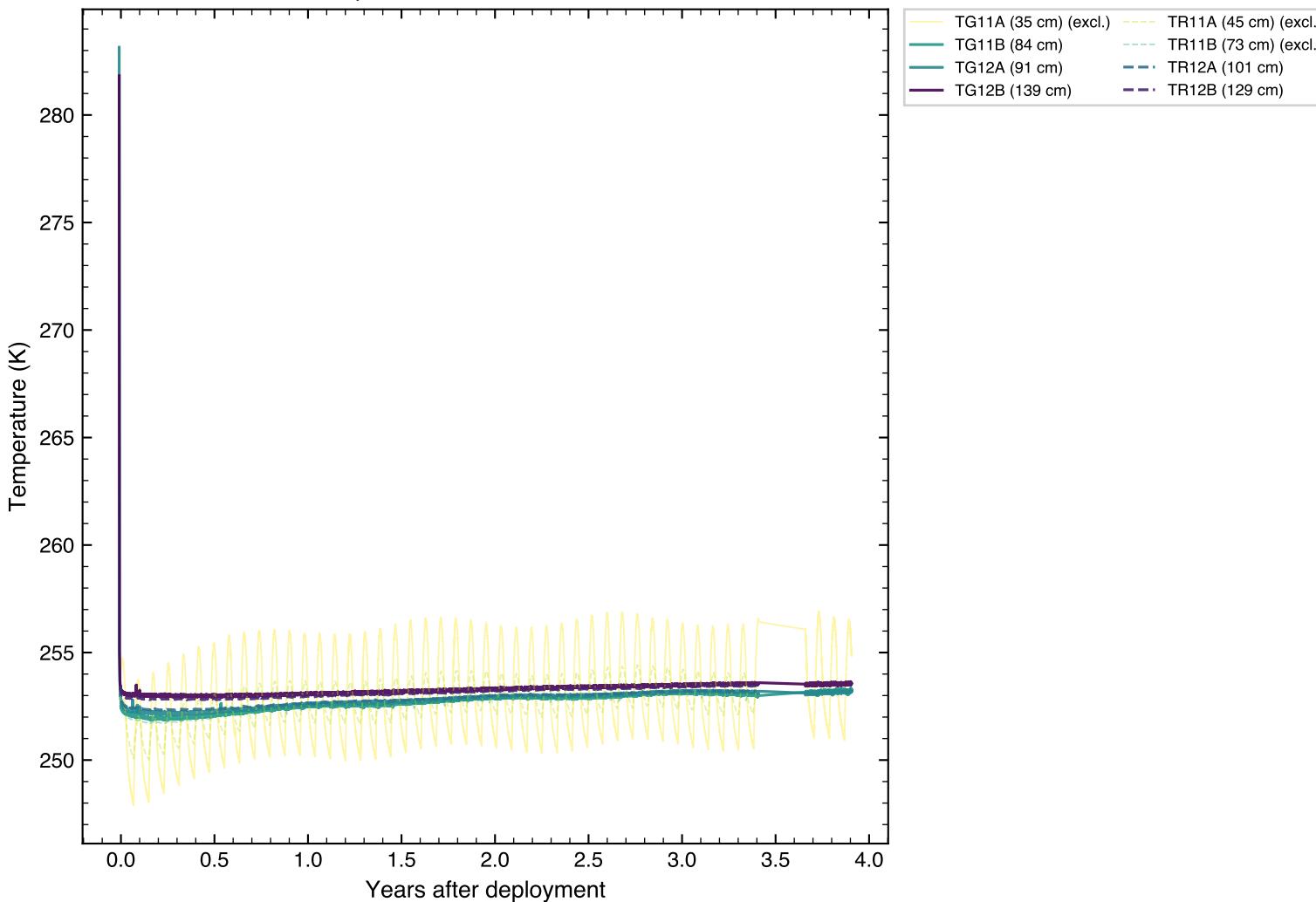
Apollo 15 HFE — Probe 1
