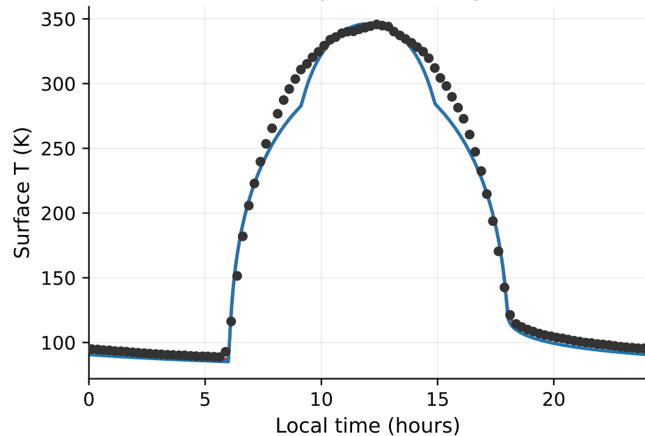
Full diurnal cycle, 45° N highlands
