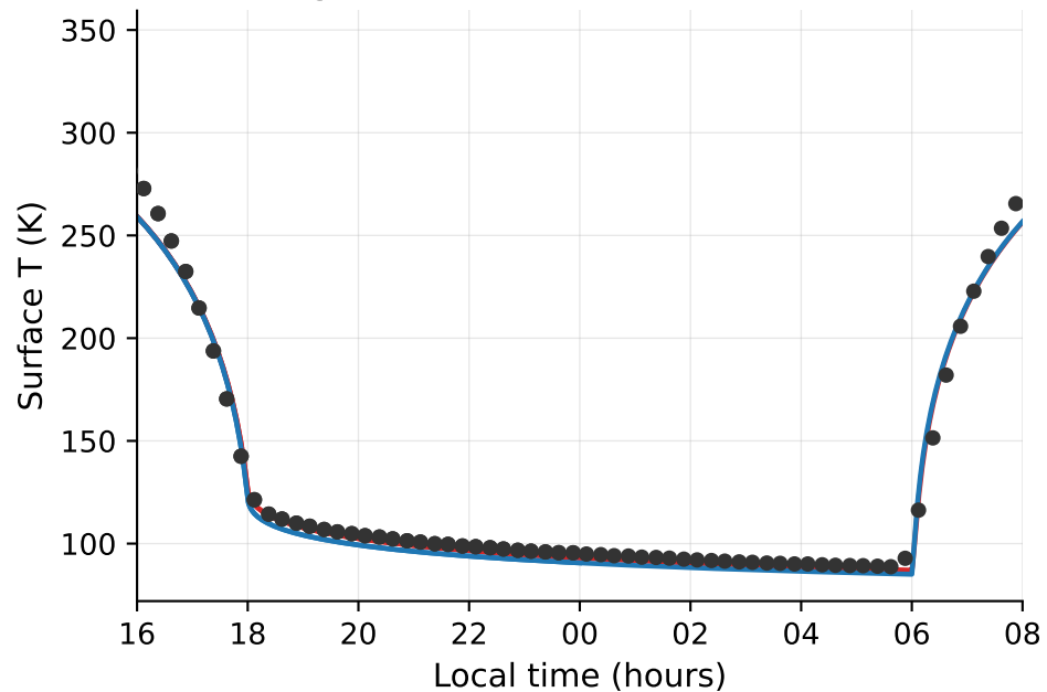
Nighttime zoom (LT 16:00 – 08:00)
