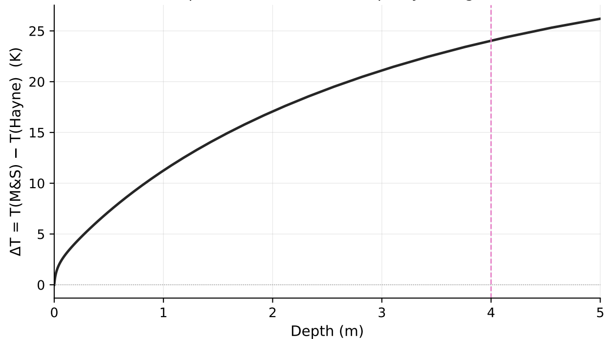
K-model \Delta T vs depth at Shoemaker (1-D proxy for Fig 9 of M&S 2021)
