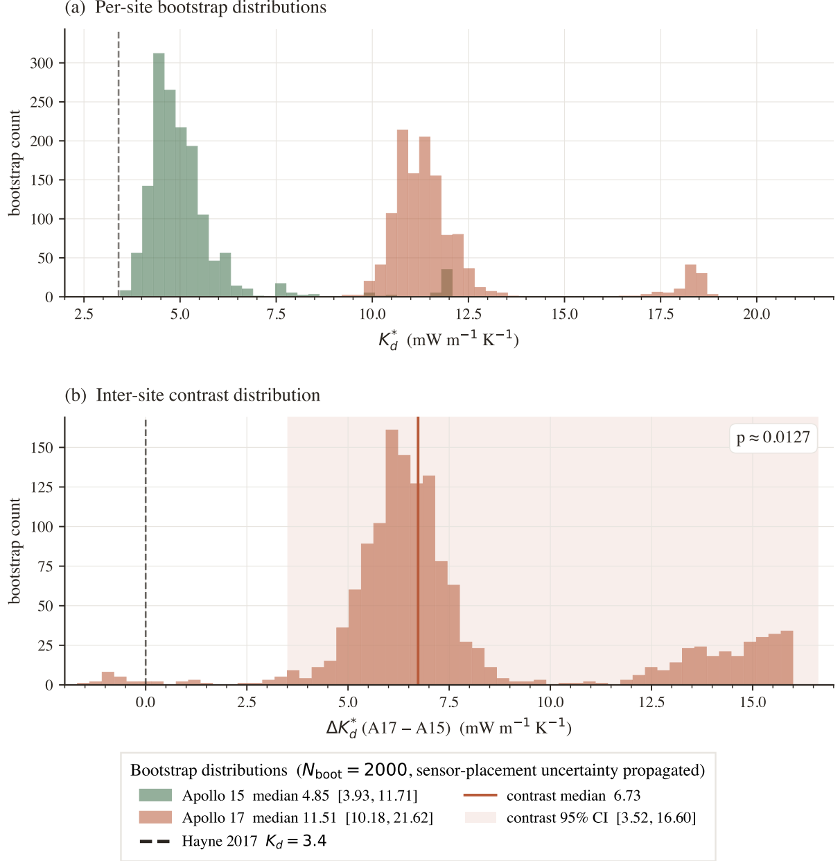
Figure 5. Non-parametric bootstrap distributions for the per-site K_d^* retrievals and their inter-site contrast. (a) Bootstrap histograms of K_d^* from N_{\text{boot}} = 2000 resamples of the deep-sensor set at each site (with replacement and with the published \pm 2.5 cm sensor-placement uncertainty propagated). The 95% confidence intervals are listed in the legend. The vertical dashed line marks the published global value K_d = 3.4 \text{ mW}/(\text{m K}) . (b) Distribution of the inter-site contrast \Delta K_d^* = K_{d,A17}^* - K_{d,A15}^* , with the 95% bootstrap CI shaded. The distribution does not overlap zero, giving p \approx 0.013 for the null of inter-site equality.
