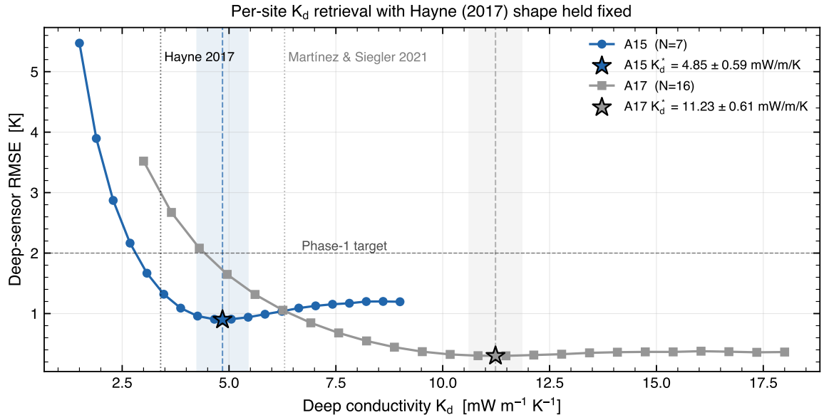
Figure 4. Per-site K_d retrieval under the Hayne et al. (2017) functional form. Deep-sensor RMSE (eq. 8) as a function of K_d , with K_s , H , \chi , T_{\text{ref}} , \rho(z) and c_p(T) all held at their published values. Filled markers are the swept grid; the solid curve is the parabolic refinement through the three values bracketing the minimum; and the shaded band is the bootstrap 95% confidence envelope. Vertical dashed lines mark the published Hayne et al. (2017) value (3.4 mW/(m K)) and the Martínez and Siegler (2021) 3-layer deep value (6.3 mW/(m K)). The two landing-site optima differ by approximately 6.7 mW/(m K), with a 95% bootstrap CI that excludes zero (Fig. 5).
