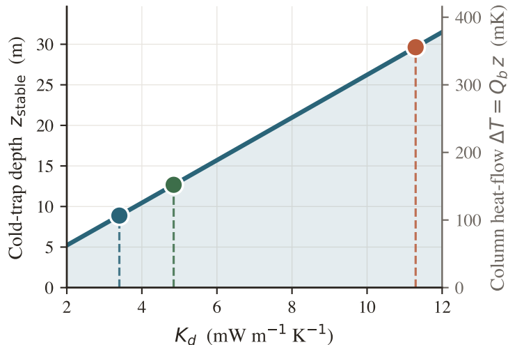
(a) Depth where buried ice is thermally stable
