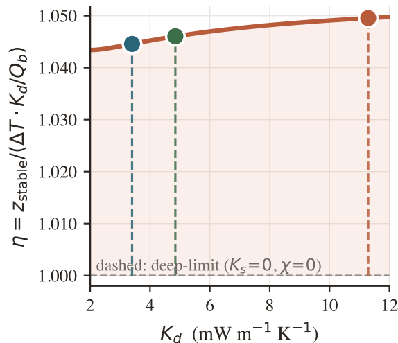
(b) Deviation from the constant- K Fourier limit
