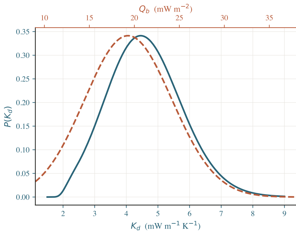
(c) A15 marginal posteriors
