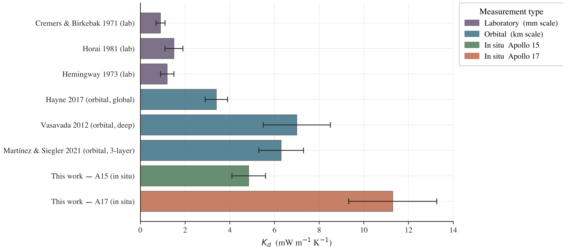
K_d estimates across measurement scales
