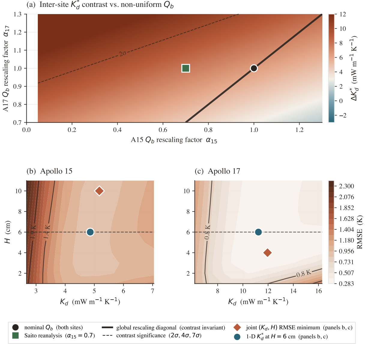
Figure 6. Robustness of the per-site K_d^* contrast. (a) Contrast \Delta K_d^* as a function of per-site Q_b rescaling factors \alpha_{15}, \alpha_{17} . Solid diagonal: global rescaling (contrast invariant); dashed contours: bootstrap- \sigma significance; black circle: nominal Q_b ; green square: Saito et al. (2007) A15 reanalysis. (b),(c) Joint (K_d, H) RMSE surface at each site over the swept H = 1\text{--}11 cm range; the coral diamond marks the joint RMSE minimum and the teal circle the 1-parameter retrieval at H = 6 cm. The RMSE surface is extremely flat in H — it varies by < 0.02 K across H = 3\text{--}11 cm — so H is effectively unconstrained, with shallow interior minima at H \approx 10 cm (A15) and 4 cm (A17). The retrieved K_d is nonetheless stable: the joint minimum and the 1-D retrieval agree in K_d to within the 0.5 K RMSE contour, confirming that K_d , not H , is the identified parameter.
