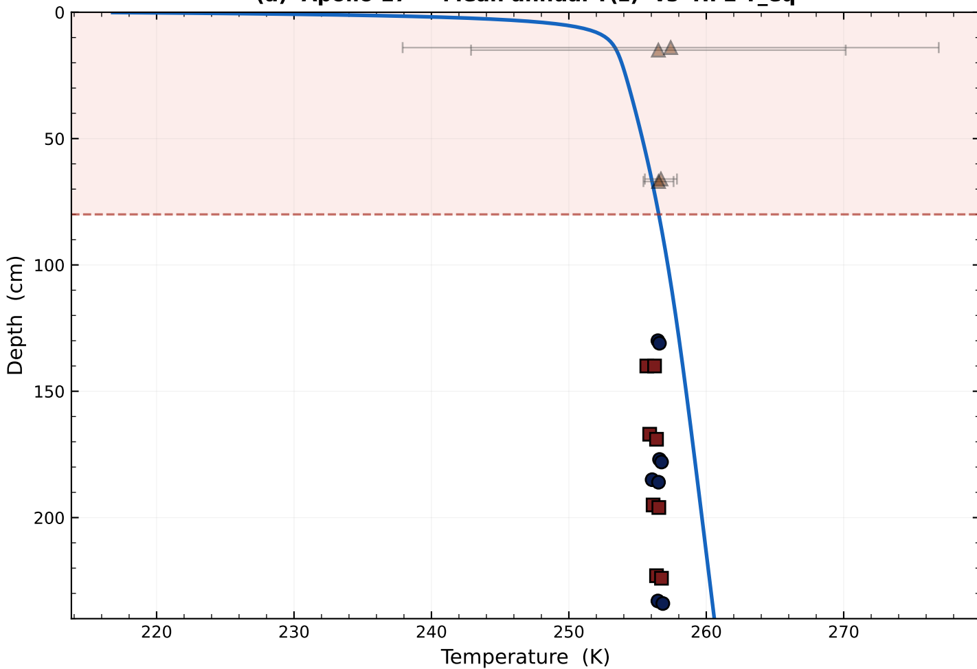
(a) Apollo 17 — Mean annual T(z) vs HFE T_{eq}
