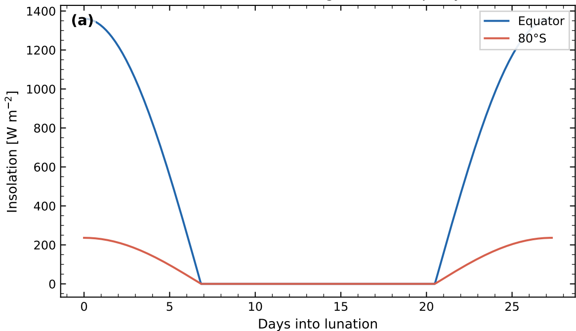
Solar insolation forcing (sinusoidal proxy)
