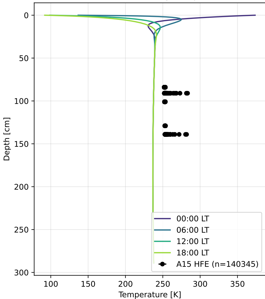
Hayne 2017 Fig. 4 — Apollo 15 reproduction (Lunar-V2 Phase 1, angle-dep albedo)
