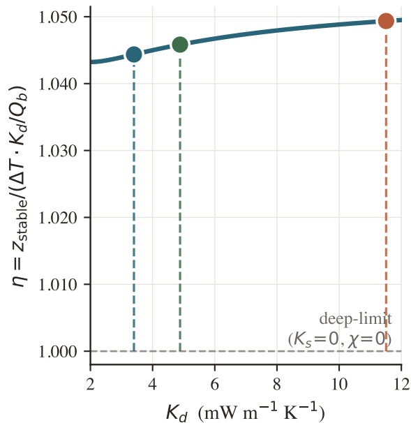
(b) Deviation from the constant- K Fourier limit
