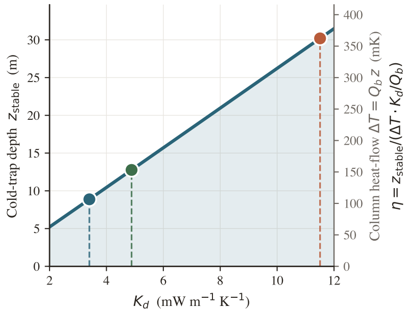
(a) Depth where buried ice is thermally stable
