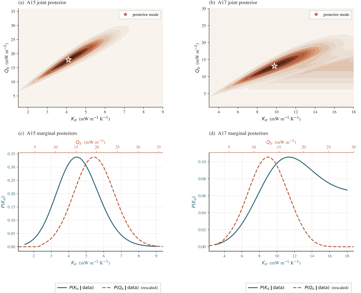
Figure 9. Joint (K_d, Q_b) posteriors and marginal distributions at each Apollo site, with the Saito–Nagihara Q_b prior propagated. (a),(b) Joint posterior density on the (K_d, Q_b) plane at Apollo 15 and Apollo 17, evaluated over the full prior-supported Q_b range so that the contour distribution fills the panel. White contours mark the 5%, 32%, and 68% mass levels; the coral star is the posterior mode; thin dotted white rays trace the iso-ratio degeneracy lines Q_b/K_d = \text{const} along which the steady-state likelihood is invariant. (c),(d) Marginal posteriors P(K_d | \text{data}) (teal solid, bottom axis) and P(Q_b | \text{data}) (coral dashed, top axis, rescaled to the P(K_d) peak). The marginal posterior medians are K_{d,A15} = 3.9 and K_{d,A17} = 13.1 \text{ mW}/(\text{m K}) , giving a paired-draw contrast probability P(K_{d,A17} > K_{d,A15}) \approx 96\% . The distribution-level inter-site contrast complements the bootstrap-based contrast in Fig. 6.
