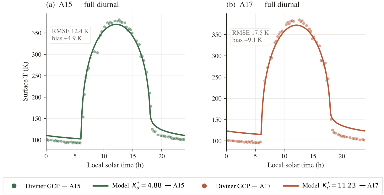
Figure 8. Surface-temperature closure against the Diviner Lunar Radiometer Global Cumulative Product. Modelled surface temperature (solid lines) at Apollo 15 (teal) and Apollo 17 (coral), run with the per-site retrieved K_d^* , overlaid on the Diviner Williams et al. (2017) diurnal brightness-temperature composite (markers). Terminator timing, daytime plateau width, and night-time floor are faithfully reproduced at both sites (full-cycle RMSE 12.4 K and 17.5 K at A15 and A17 respectively); the model runs slightly warmer than the Diviner composite across the full cycle, with the largest discrepancy on the night side, consistent with the well-documented anisothermal-footprint and sub-pixel rock-population effects (Bandfield et al., 2015; Hayne et al., 2017) and does not affect the deep-gradient retrieval.
