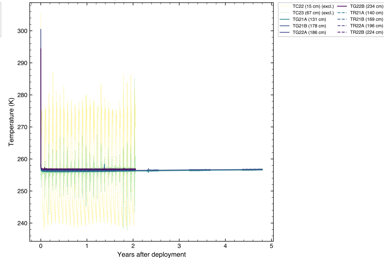
Apollo 17 HFE — Probe 2
