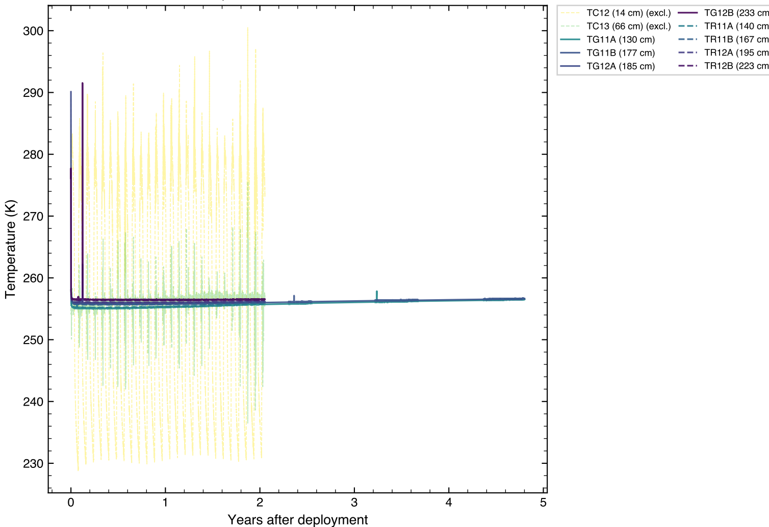
Apollo 17 HFE — Probe 1
