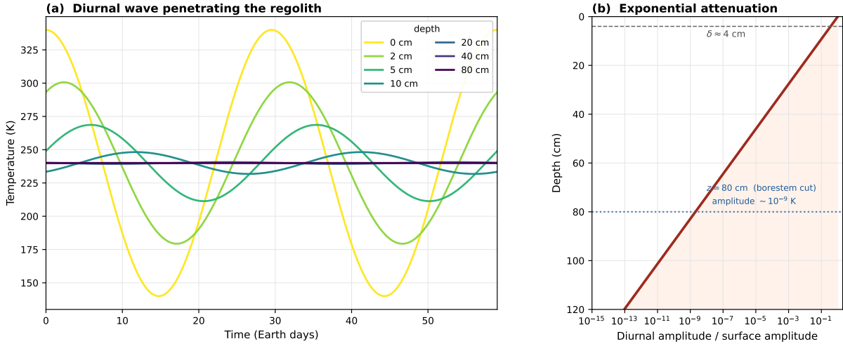
Figure 2.1. Diurnal-wave attenuation in the lunar regolith. (a) Two lunations of synthetic surface-driven temperature at selected depths; the surface (yellow) sees the full \sim 200 K peak-to-peak diurnal swing while sensors at 40 cm and below show an essentially flat trace. (b) The corresponding amplitude attenuation factor \exp(-z/\delta) on a logarithmic axis, with the e-folding skin depth \delta \approx 4 cm and the borestem-cut threshold 80 cm marked. Below 80 cm the residual diurnal amplitude \sim 10^{-9} K is many orders of magnitude below the digitisation noise floor of the restored 1971–1977 record ( \sim 0.05 – 0.2 K).
