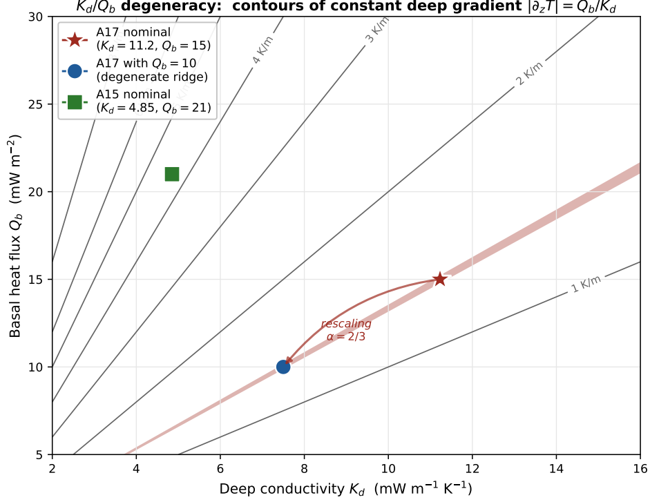
Figure 4.1. The K_d/Q_b degeneracy of single-borehole inversions. Grey contours show curves of constant deep equilibrium gradient |\partial_z T| = Q_b/K_d . The Apollo 17 retrieval (red star) and the Apollo 15 retrieval (green square) sit on different contours, confirming that the inter-site contrast is not a Q_b artefact. The blue circle shows where the A17 retrieval would move if the basal heat flux were closer to the Saito et al. (2007) ; Nagihara et al. (2018) reanalysis value of \sim 10 \text{ mW/m}^2 : the rescaling ( \alpha = 2/3 , red arrow) slides the retrieval along the same iso-gradient ridge from (K_d, Q_b) = (11.2, 15) to (K_d, Q_b) = (7.5, 10) . Crucially, this rescaling does not change the equilibrium temperature profile, and so it is invisible to a single-borehole inversion.
