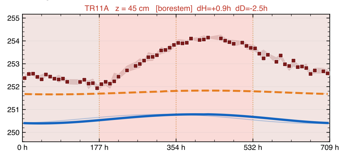
Apollo 15 HFE — Diurnal Cycle Comparison (SPICE LST) Peak-aligned model vs Apollo binned medians (lat = 26.13°N)
