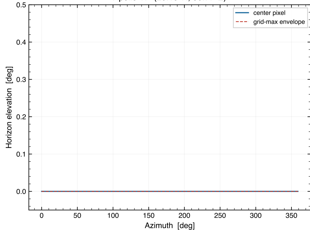
Fig 9 — Synthetic flat-plain horizon at the Apollo sites (max < 0.05° □ flat-terrain assumption verified)
