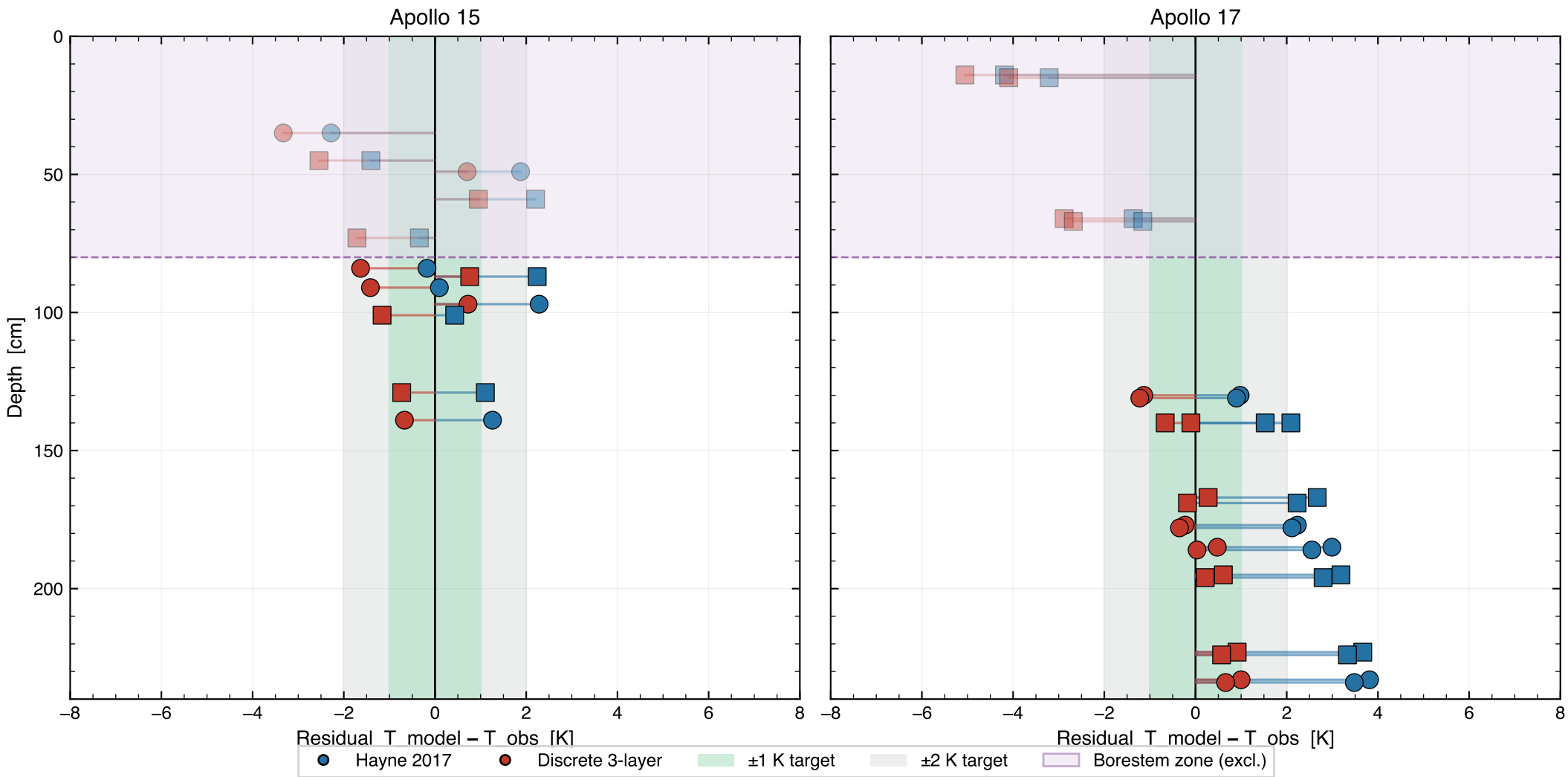
Fig 6 — Residual T(\text{model}) - T(\text{obs}) versus depth
