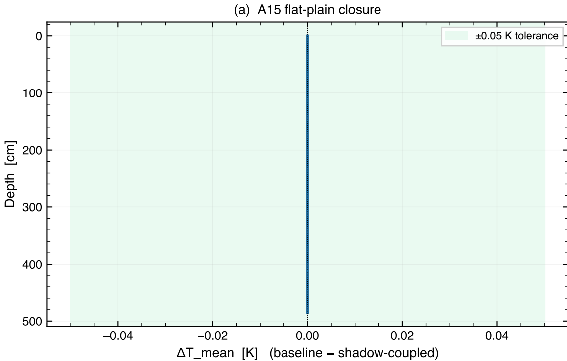
Fig 14 — Shadow mask hooked into solve_pixel Flat-plain closure: \max|\Delta T| = 0.0000 K (PASS < 0.05 K)
