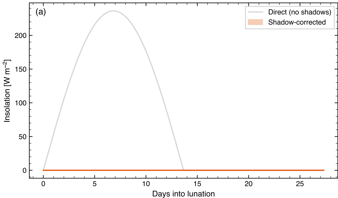
Crater center: direct vs shadow-corrected insolation
